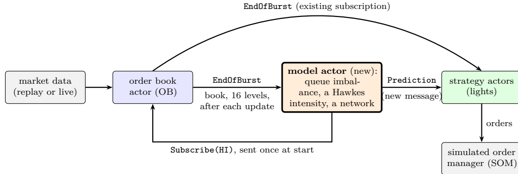
Figure 84: An order-book model added to Kaspar as an actor. It subscribes to the order book, receives the book after each burst of updates, and sends a prediction message to each strategy actor. Message names are those in the code; the model actor, the Prediction message and its handler in the strategy are new.
