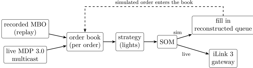
Figure 83: Kaspar data and order paths. Everything downstream of the market-data source is the same code in replay and live operation; the branch between simulated and live execution is a single decision in the simulated order manager.
