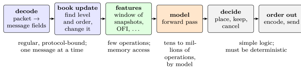
Figure 85: The per-event pipeline of a model-driven trading system. The model stage is the only one whose cost depends on the modeller’s choices. Schematic.
