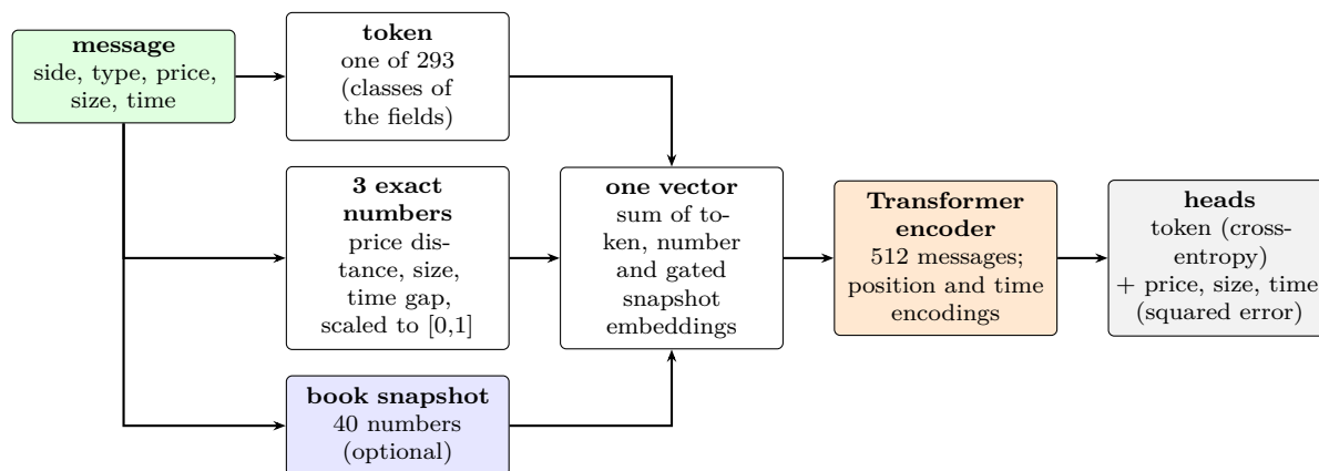
Figure 78: LOBERT’s pipeline: each message becomes one token plus three exact numbers, optionally with the book snapshot after it; these are combined into one vector per message, passed through a Transformer encoder that is aware of the time between messages, and decoded by a token head and three number heads. After Linna et al. (2025).
