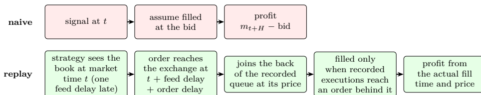
Figure 81: A naive backtest and a queue-exact replay of the same passive order. The naive backtest fills the order as soon as the signal fires; the replay sends it with its delays, places it in the recorded queue and fills it only when the recorded executions reach it.
