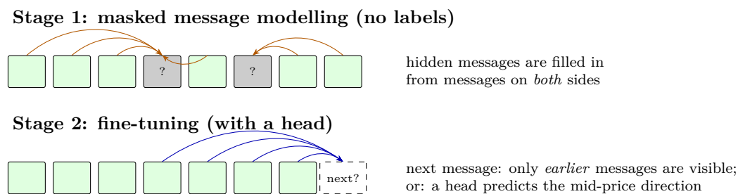
Figure 79: LOBERT’s two training stages. Stage 1 hides random messages (grey) and learns to reconstruct them from both sides; stage 2 starts from those weights and trains for a task, with a causal mask for next-message prediction or a classification head for mid-price direction. Schematic.
