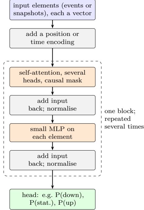
Figure 70: A Transformer. Each block mixes information across elements (self-attention) and then transforms each element on its own (MLP); blocks are stacked. Schematic.
