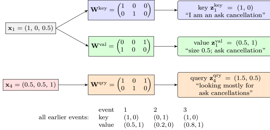
Figure 73: Step 2: each event’s embedding is multiplied by three learned matrices. The earlier events supply keys and values (top, for event 1; the table lists all three). The current event supplies the query (bottom). Example: \mathbf{W}^{\text{key}}\mathbf{x}_1 = (1 \cdot 1 + 0 \cdot 0 + 0 \cdot 0.5, 0 \cdot 1 + 1 \cdot 0 + 0 \cdot 0.5) = (1, 0) .
