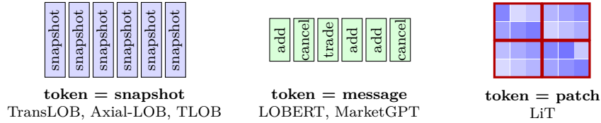
Figure 71: Three ways to cut order-book data into the tokens a Transformer attends over. Schematic.
