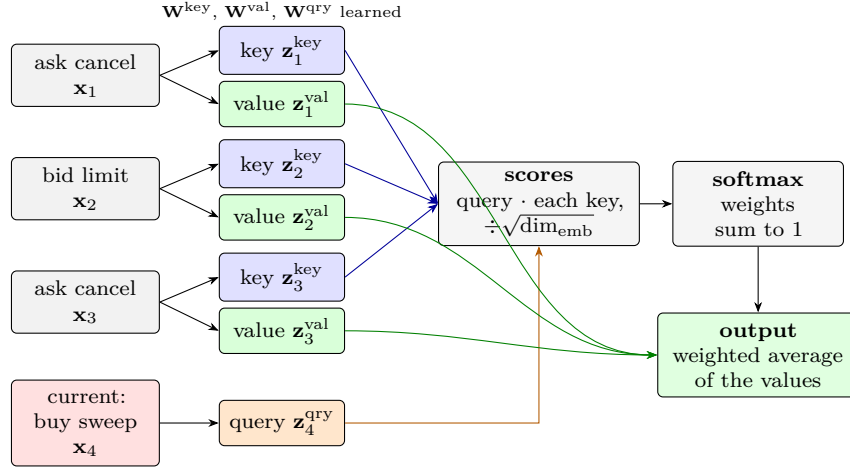
Figure 75: The attention step on order-book events. Each event's embedding is turned into a key and a value (earlier events) and a query (current event) by three learned matrices; the query is scored against each key, the scores are turned into weights, and the output is the weighted average of the values. Schematic.
