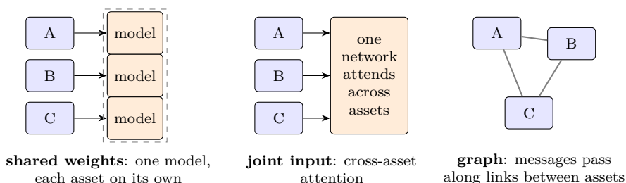
Figure 80: Three ways deep models connect several assets. Schematic.
