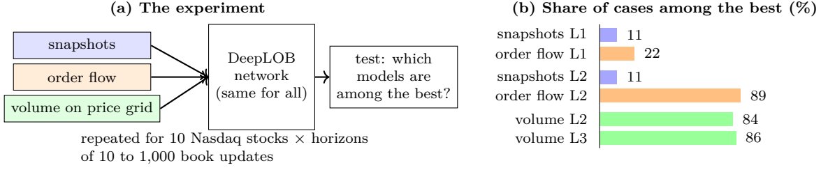
Figure 50: The input experiment of Lucchese et al. (2024) . (a) Only the input changes; the network is fixed. “Among the best”: not shown to be worse than the best model by a model confidence set test at the 1% level. (b) Share of (stock, horizon) cases in which each input was among the best, stock-specific models (their Table 5). L1, L2, L3: the paper’s labels for variants of each input. Several inputs can be among the best in the same case, so the shares do not sum to 100%.
