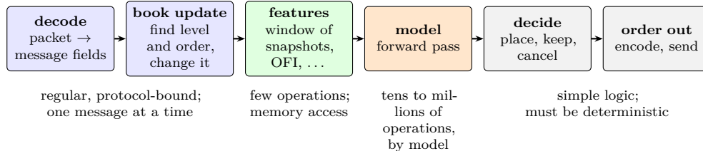
Figure 80: The per-event pipeline of a model-driven trading system. The model stage is the only one whose cost depends on the modeller’s choices. Schematic.
