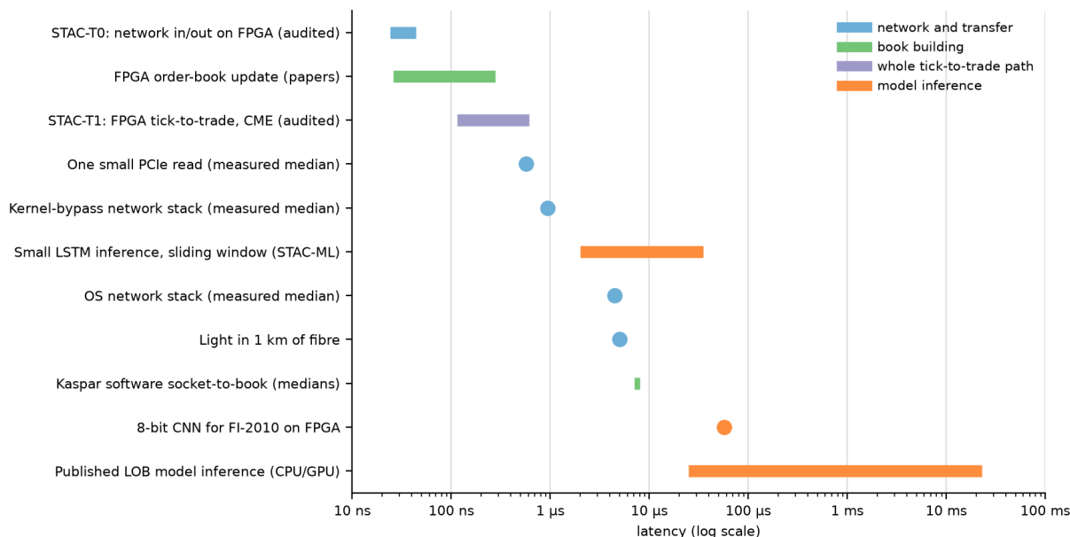
Figure 81: Latency figures quoted in this section, on one logarithmic axis. Bars are ranges, dots single figures. Sources: STAC public summaries (audited), the FPGA book-building papers, the measured server latency budget (Zilberman et al., 2017), Kaspar’s published socket-to-book medians (Maciejewski, 2026c), and Table 55. The figures come from different machines, conditions and years and show orders of magnitude, not a single system.
