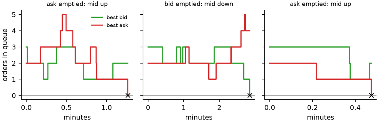
Figure 2: Three simulated races between the best-bid and best-ask counters, each starting from 3 orders at the bid and 2 at the ask, with the estimated rates of Table 8 at distance one. Each step up is a limit order joining; each step down is a market order or a cancellation. The race ends (cross) when one counter reaches zero, and that side decides the next price move. The same starting book can end either way, and after very different waiting times: the model’s answers are probabilities. Stylised simulation for illustration; not data.
