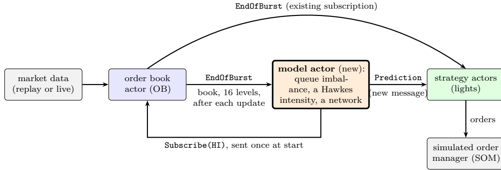
Figure 79: An order-book model added to Kaspar as an actor. It subscribes to the order book, receives the book after each burst of updates, and sends a prediction message to each strategy actor. Message names are those in the code; the model actor, the Prediction message and its handler in the strategy are new.
