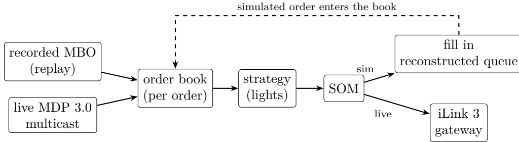
Figure 78: Kaspar data and order paths. Everything downstream of the market-data source is the same code in replay and live operation; the branch between simulated and live execution is a single decision in the simulated order manager.
