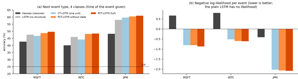
Figure 39: Results reported by Shi and Cartlidge (2022) , Table 1, re-plotted; not our data. (a) Accuracy of predicting the type of the next event, with the time of the event given; dashed line: guessing among four types. (b) Negative log-likelihood per event; the plain LSTM has no likelihood.
