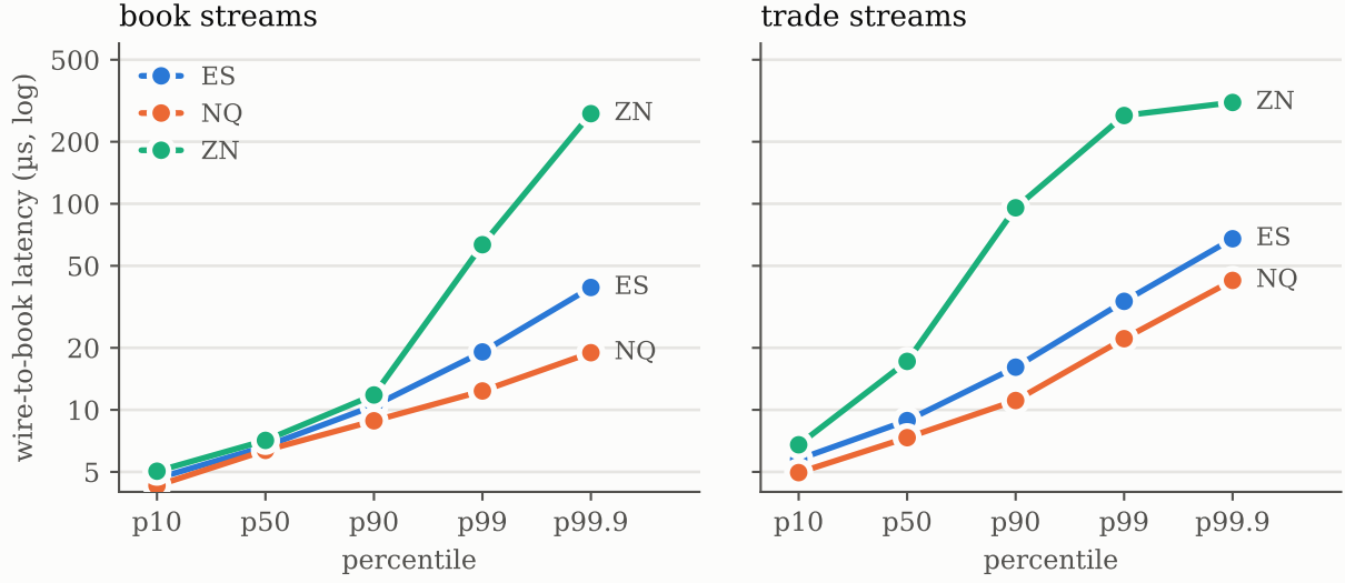
Figure 4. Serial wire-to-book latency by percentile on the six live streams, one 900 s window each, recovery excluded (book streams left, trade streams right, log latency axis). The tails order by messages per packet and cost per message, not by packet rate: the busiest stream (NQ book) has the smallest tail.
