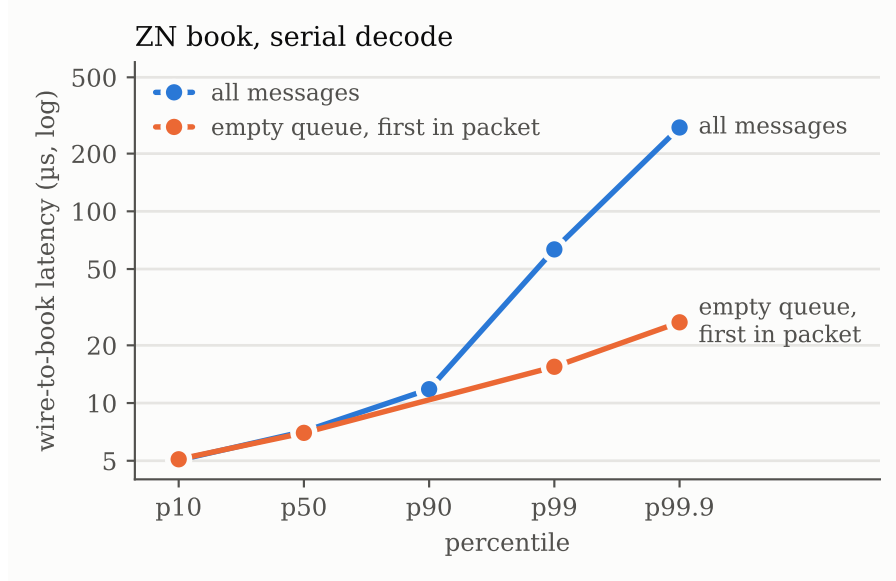
Figure 3. Wire-to-book latency by percentile on the ZN book stream, serial decode, for every message and for the hot path alone (empty queue, first in packet; its p_{90} was not reported). Log latency axis. The two populations share a floor near 5\text{--}7\ \mu\text{s} and separate only in the tail: the hot path reaches 26\ \mu\text{s} at p_{99.9} , all messages 274\ \mu\text{s} .
