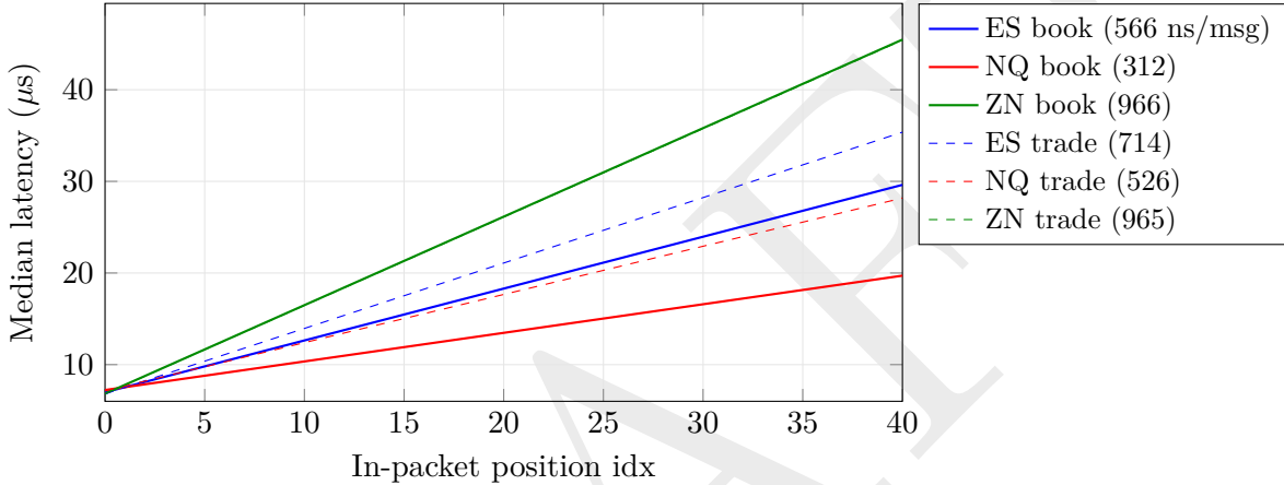
Figure 3. The per-message model median = floor + slope \times idx (Table 7), one line per stream. All six share a \sim 7 \mu\text{s} floor at idx = 0; the slope — the per-message serialization cost — sets the divergence, from 312 ns/msg (NQ book) to 966 ns/msg (ZN book).
