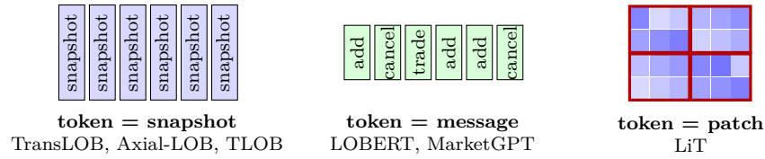
Figure 69: Three ways to cut order-book data into the tokens a Transformer attends over. Schematic.
