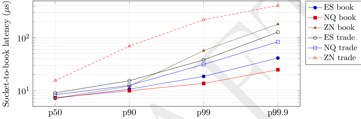
Figure 4. Socket-to-book latency percentiles per stream (Table 10), log scale. Medians cluster near 7–15 \mu\text{s} ; the tails diverge, ZN trade reaching 219 \mu\text{s} at p99 and 410 \mu\text{s} at p99.9 .
