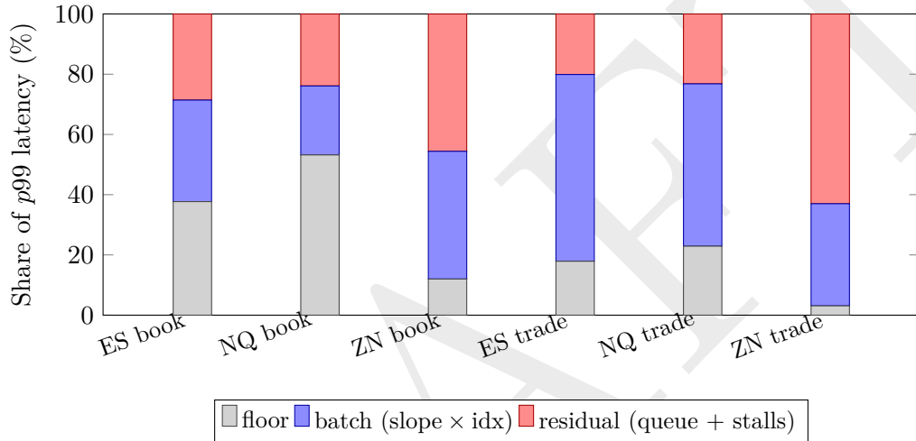
Figure 5. The tail is not the floor. Composition of each stream’s p99 socket-to-book latency: the floor, the in-packet batch ( slope \times idx evaluated at the p99 position), and the residual (queue and stalls); absolute p99 ranges from 13.6 to 219.4 \mu s (Table 18). The floor — decode, book, and the actor framework — is a minority of the tail and falls to 3–12% on the worst streams (ZN); the structured growth is the batch term. The queue, which fires on 0.08% of messages, is only a small part of the residual; the remainder is the stall population.
