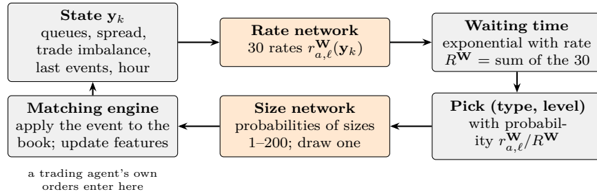
Figure 39: One step of the multidimensional deep queue-reactive simulator. Grey: the classical queue-reactive mechanism, unchanged (Figure 13). Orange: the two parts learned by networks. The paper reports 0.037 ms per generated event for the networks, excluding the matching engine.
