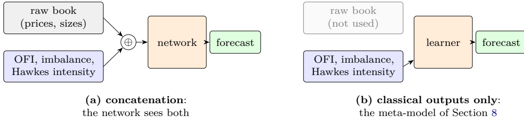
Figure 44: Concatenation. (a) The classical outputs ( \oplus : placed side by side) are extra inputs next to the raw book. (b) Remove the raw book and the same design is a meta-model. Comparing (a) with a network on the raw book alone is the ablation of Example 9.1. Schematic.
