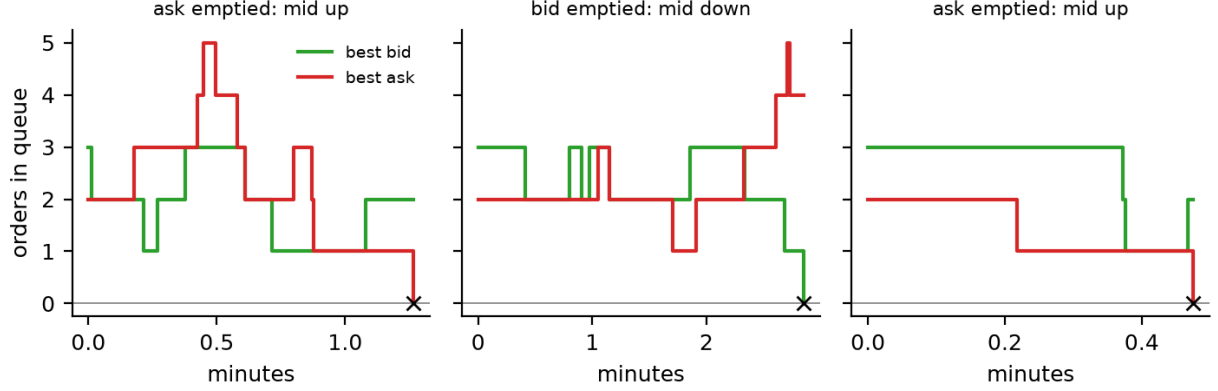
Figure 4: Three simulated races between the best-bid and best-ask counters, each starting from 3 orders at the bid and 2 at the ask, with the estimated rates of Table 10 at distance one. Each step up is a limit order joining; each step down is a market order or a cancellation. The race ends (cross) when one counter reaches zero, and that side decides the next price move. The same starting book can end either way, and after very different waiting times: the model’s answers are probabilities. Stylised simulation for illustration; not data.
