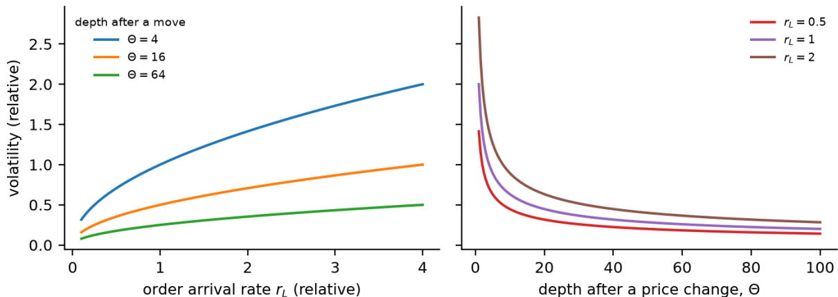
Figure 11: Cont-de Larrard model: volatility \propto \delta \sqrt{r_L / \Theta} , in relative units, against the order arrival rate for three depths (left) and against the depth after a price change for three arrival rates (right). Busier markets are more volatile; markets that refill deeply after each move are calmer.
