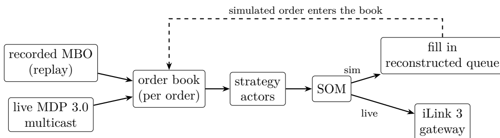
Figure 85: Kaspar data and order paths. Everything downstream of the market-data source is the same code in replay and live operation; the branch between simulated and live execution is a single decision in the simulated order manager.
