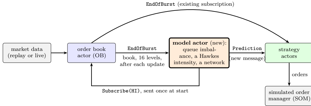
Figure 86: An order-book model added to Kaspar as an actor. It subscribes to the order book, receives the book after each burst of updates, and sends a prediction message to each strategy actor. Message names are those in the code; the model actor, the Prediction message and its handler in the strategy are new.
