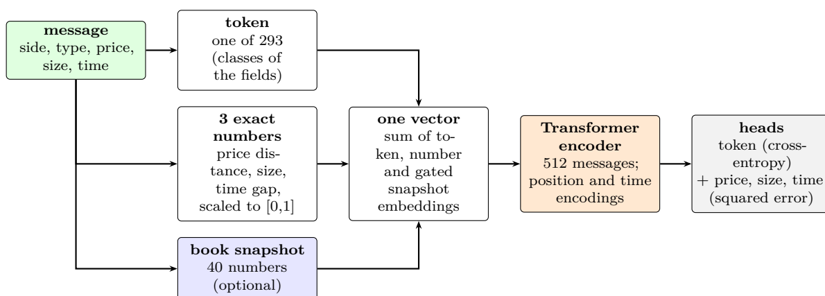
Figure 80: LOBERT’s pipeline: each message becomes one token plus three exact numbers, optionally with the book snapshot after it; these are combined into one vector per message, passed through a Transformer encoder that is aware of the time between messages, and decoded by a token head and three number heads. After Linna et al. (2025).
