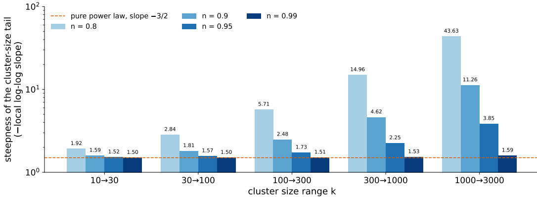
Figure 35. Table 30 as bars, log scale: how steeply the cluster-size distribution falls over successive size ranges, for four branching ratios. Near criticality ( n = 0.99 ) it keeps the power-law slope of 3/2 (dashed) over the whole range; at n = 0.8 it falls off exponentially beyond about 25, so very large clusters are rare.
