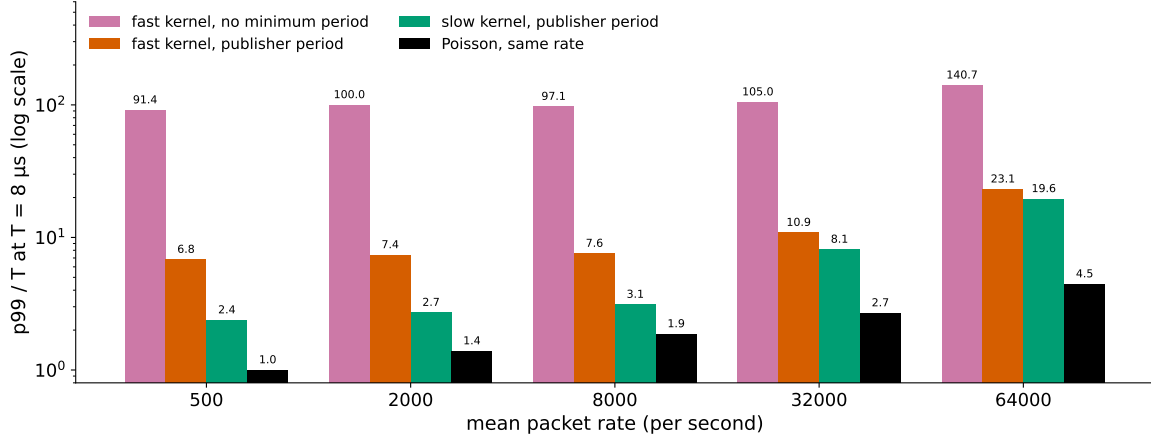
Figure 36. Table 31 as bars, log scale, for branching ratio 0.8: the normalised tail p_{99}/T at T = 8 \mu s on synthetic feeds, by packet rate. A fast kernel with no minimum period (pink) has a tail of about a hundred times T ; adding a minimum period equal to the publisher period (vermillion) cuts it more than tenfold; a slow kernel with the minimum period (green) is lower still, closer to the Poisson stream (black). What sets the tail at 8 \mu s is how many gaps sit at the minimum period, which the kernel and the minimum period control and the branching ratio alone does not.
