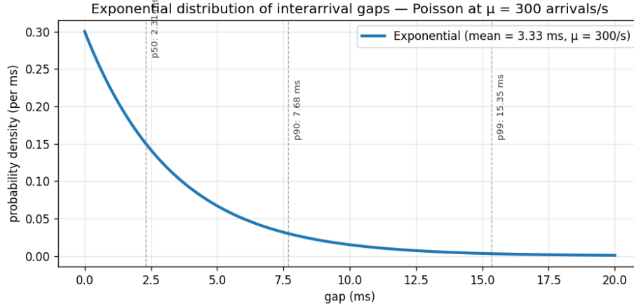
Figure 30. The exponential density of interarrival gaps for a Poisson process at 300 arrivals per second. Dashed vertical lines mark the median, p_{90} and p_{99} . Half the gaps are shorter than the median of 2.3 ms and 10% are longer than 7.7 ms. The CME packet stream has a different shape: far more mass near zero and a much heavier right tail (Figure 6).
