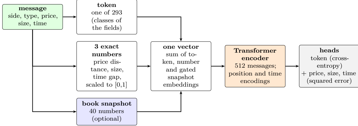
Figure 80: LOBERT’s pipeline: each message becomes one token plus three exact numbers, optionally with the book snapshot after it; these are combined into one vector per message, passed through a Transformer encoder that is aware of the time between messages, and decoded by a token head and three number heads. After Linna et al. (2025).
