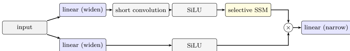
Figure 79: The Mamba block. The second branch gates the output of the selective state-space layer by multiplication. After Gu and Dao (2024).
