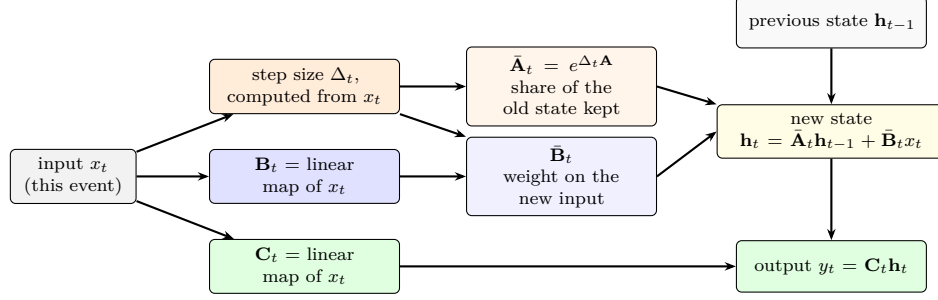
Figure 78: One step of Mamba’s selective state-space layer. The current input sets the step size \Delta_t and the matrices \mathbf{B}_t and \mathbf{C}_t ; the step size sets how much of the previous state survives. After Gu and Dao (2024).
