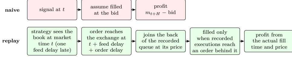
Figure 83: A naive backtest and a queue-exact replay of the same passive order. The naive backtest fills the order as soon as the signal fires; the replay sends it with its delays, places it in the recorded queue and fills it only when the recorded executions reach it.
