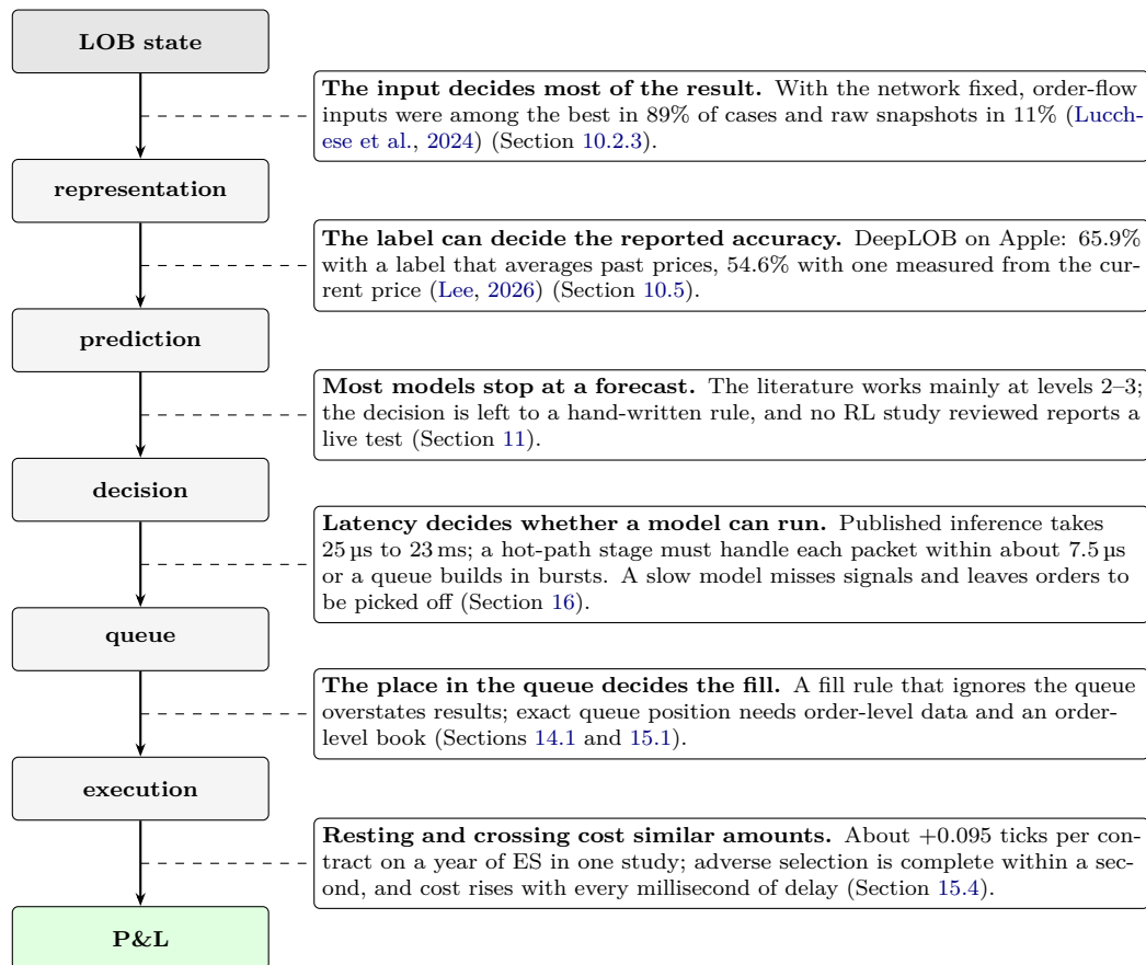
Figure 89: The chain from order book to profit, with what the survey found at each link and where. Figures are those quoted in the sections named, with their sources there.
