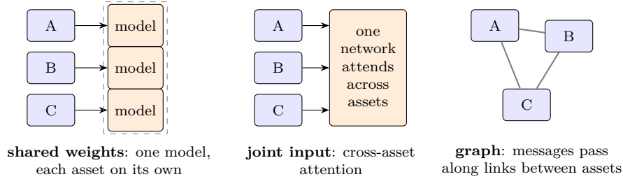
Figure 82: Three ways deep models connect several assets. Schematic.
