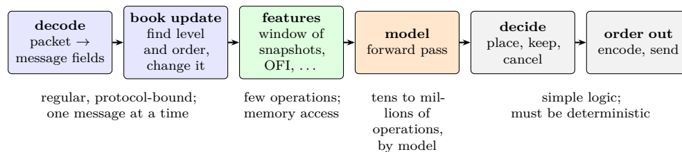
Figure 87: The per-event pipeline of a model-driven trading system. The model stage is the only one whose cost depends on the modeller’s choices. Schematic.
