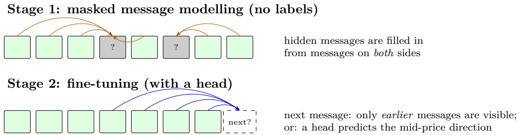
Figure 81: LOBERT’s two training stages. Stage 1 hides random messages (grey) and learns to reconstruct them from both sides; stage 2 starts from those weights and trains for a task, with a causal mask for next-message prediction or a classification head for mid-price direction. Schematic.
