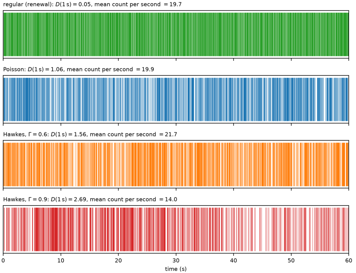
Figure 21: Four simulated processes with a mean rate of about 20 per second, over 60 seconds. Top: a renewal process with very regular gaps (gamma-distributed with shape 25), D(1\text{ s}) \approx 0.05 : nearly equal counts per window. Second: Poisson, D \approx 1 , the reference. Third: Hawkes with \Gamma = 0.6 , D(1\text{ s}) \approx 1.6 : visible clumping. Bottom: Hawkes with \Gamma = 0.9 , D(1\text{ s}) \approx 2.7 : pronounced bursts and long quiet stretches. Redrawn after Maciejewski (2026b); stylised simulation.
