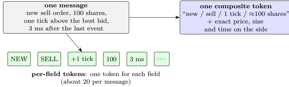
Figure 77: Two ways of tokenising the same message. Field-level schemes ( Nagy et al., 2023 ) emit one token per field; event-level schemes ( Linna et al., 2025 ) map the whole event to a single token from a vocabulary of binned combinations, and may pass the exact values alongside. Schematic.
