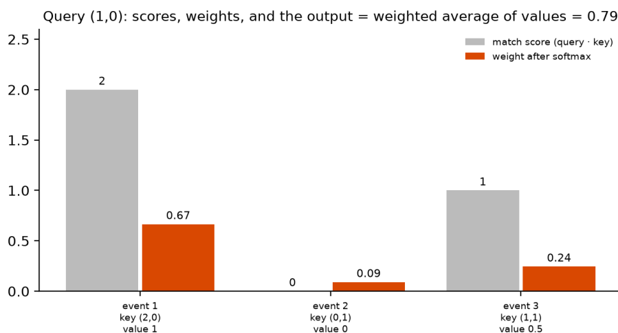
Figure 63: The worked example above. Grey: the match score of the query (1,0) with each key. Orange: the weights the softmax turns the scores into. The output is the weighted average of the values, 0.79. Illustrative numbers.
