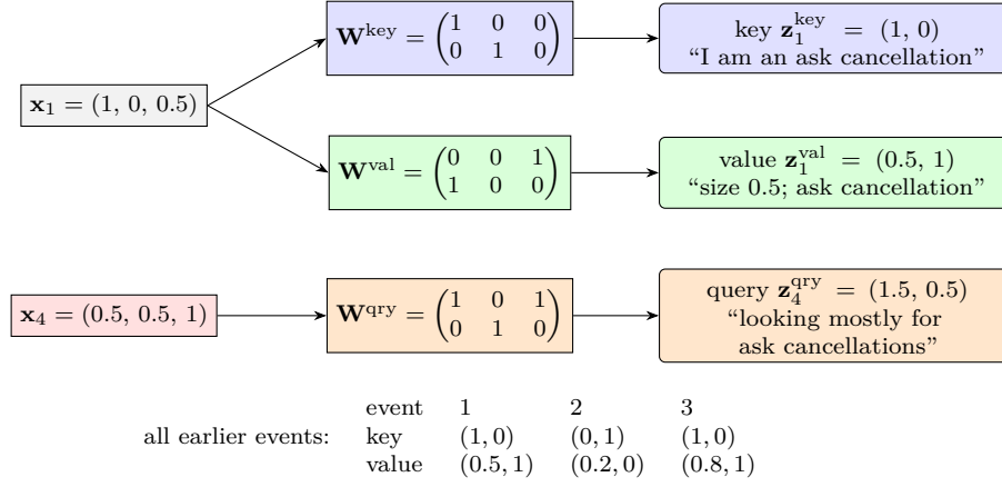
Figure 69: Step 2: each event’s embedding is multiplied by three learned matrices. The earlier events supply keys and values (top, for event 1; the table lists all three). The current event supplies the query (bottom). Example: \mathbf{W}^{\text{key}} \mathbf{x}_1 = (1 \cdot 1 + 0 \cdot 0 + 0 \cdot 0.5, 0 \cdot 1 + 1 \cdot 0 + 0 \cdot 0.5) = (1, 0) .
