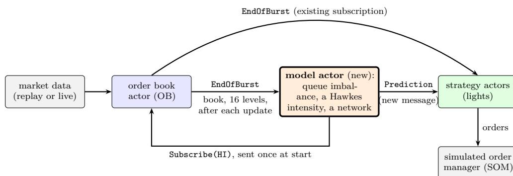
Figure 84: An order-book model added to Kaspar as an actor. It subscribes to the order book, receives the book after each burst of updates, and sends a prediction message to each strategy actor. Message names are those in the code; the model actor, the Prediction message and its handler in the strategy are new.
