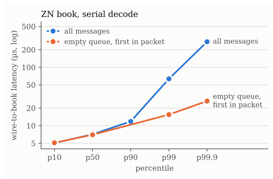
Figure 28. Wire-to-book latency by percentile on the ZN book stream, serial decode, for every message and for the empty-queue messages alone (empty queue, first in packet; its p_{90} was not reported). Log latency axis. The two populations share a minimum near 5–7 \mu\text{s} and separate only in the tail: the empty-queue messages reach 26 \mu\text{s} at p_{99.9} , all messages 274 \mu\text{s} .
