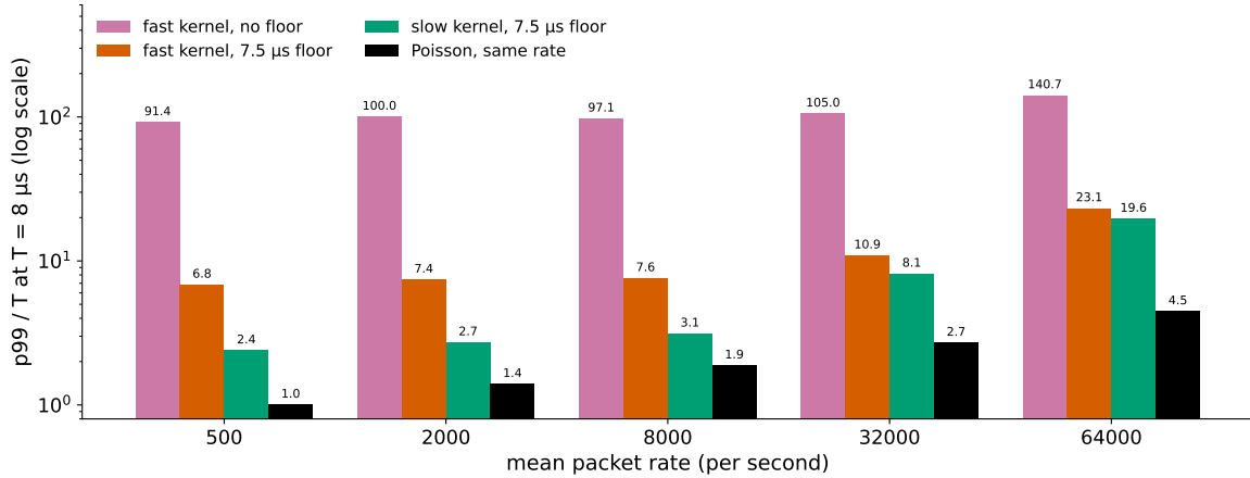
Figure 31. Table 28 as bars, log scale, for branching ratio 0.8: the normalised tail p_{99}/T at T = 8 \mu s on synthetic feeds, by packet rate. A fast kernel with no floor (pink) has a tail of about 100 times T ; adding a 7.5 \mu s floor (vermillion) cuts it more than tenfold; a slow kernel with the floor (green) is lower still, 2 to 3 times T at low rates against 1 to 2 for the Poisson stream (black). What sets the tail at 8 \mu s is how many gaps sit at or below the floor, which the kernel and the floor control and the branching ratio alone does not.
