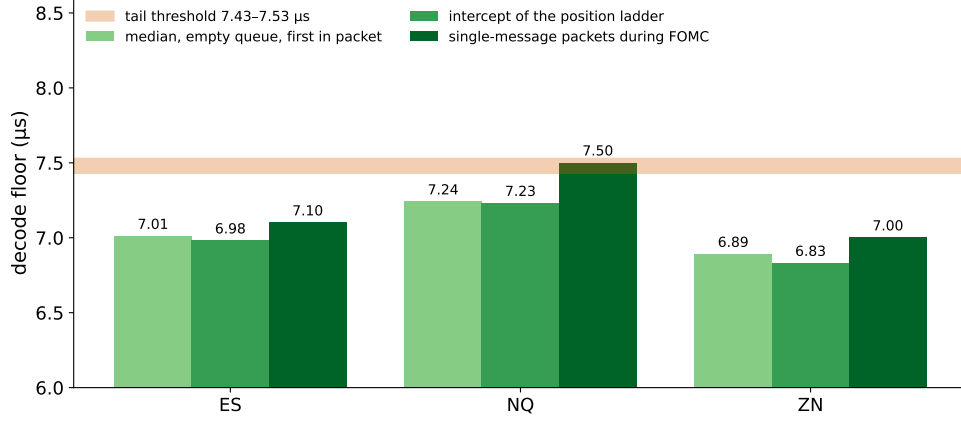
Figure 22. Table 20 as bars: the production decoder’s floor by three independent estimates on each instrument, against the tail threshold measured on the corpus (shaded band). All nine estimates lie in or just below the band: the production receiver runs right at the edge of the tail.
