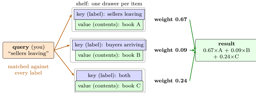
Figure 65: Attention as a library search. You bring a query; every drawer on the shelf carries a key (its label) and a value (its contents). The query is matched against every label, the matches become weights that sum to one, and you get back a mix of all the contents, mostly from the drawers that matched best. Numbers from the worked example below.
