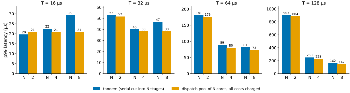
Figure 11. Table 10 as bars: p_{99} of a serial cut into N stages (blue) against a pool of N cores with the ingress hop, egress hop and resequencing charged (orange). At N = 2 the two are level; from N = 4 the pool is lower at every service time, and at 16 \mu s its p_{99} does not grow with N while the tandem’s does.
