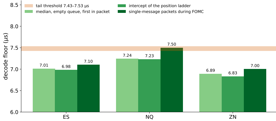
Figure 22. Table 23 as bars: the production decode floor by three independent estimates on each instrument, against the tail threshold measured on the corpus (shaded band). All nine estimates lie in or just below the band: the production receiver runs right at the edge of the tail.
