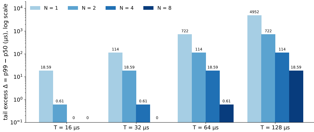
Figure 12. Table 11 as bars, log scale: the tail excess \Delta = p_{99} - p_{50} for N = 1, 2, 4 and 8 stages at each service time. Each extra split moves the excess down to the value of the next shorter service time: at T = 128 \mu\text{s} , N = 2 has the excess of a single thread at 64 , N = 4 that at 32 , and so on, because only the largest stage matters. Once the per-stage service is below the publisher spacing the excess is zero (bars marked 0).
