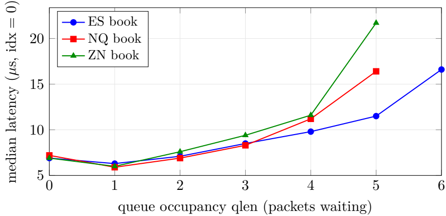
Figure 4. Latency rises with queue occupancy (two-stage configuration, 2026-09-16). Median socket-to-book latency against queue occupancy \text{qlen} for the three book streams, with in-packet position held at \text{idx} = 0 to isolate the queue from packet size. At \text{qlen} = 0 — the state 87%–99.7% of messages find — the median sits at the \sim 7 \mu\text{s} two-stage floor; each further queued packet adds more than the last (convex), so the tail, where it is queue-driven, tracks \text{qlen} . The effect is confined to a rare event ( \text{qlen} \geq 3 on 0.08% of messages). Deep-queue points ( \text{qlen} \geq 5 ) rest on few messages and are noisier.
