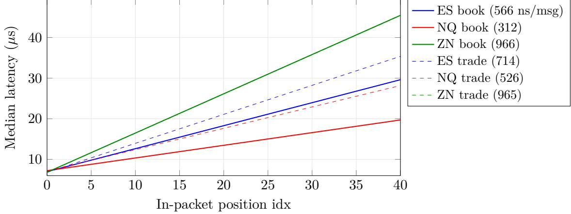
Figure 2. The per-message model median = floor + slope \times idx in the two-stage configuration (Table 9), one line per stream. All six share a \sim 7 \mu s two-stage floor at idx = 0 (it includes the cross-thread hand-off; the one-thread book-update medians are 0.8–1.1 \mu s ); the slope — the per-message serialization cost — sets the divergence, from 312 ns/msg (NQ book) to 966 ns/msg (ZN book).
