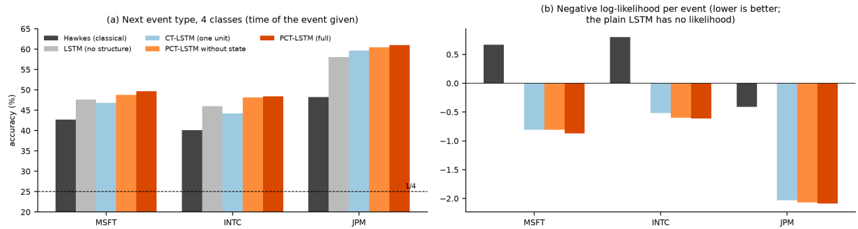
Figure 42: Results reported by Shi and Cartlidge (2022), Table 1, re-plotted; not our data. (a) Accuracy of predicting the type of the next event, with the time of the event given; dashed line: guessing among four types. (b) Negative log-likelihood per event; the plain LSTM has no likelihood.
