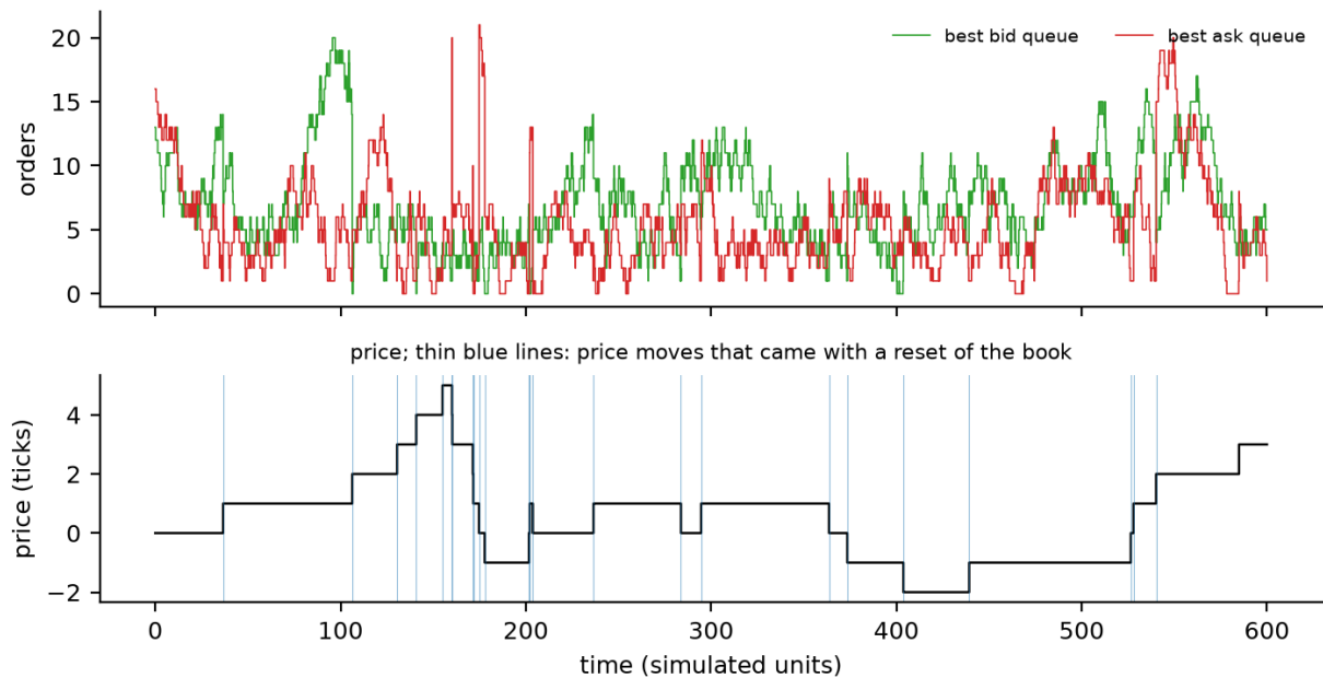
Figure 16: A run of a queue-reactive simulator with two levels per side, rate functions of the shapes in Figure 15 scaled to short queues, \pi_{\text{move}} = 0.7 and \pi_{\text{reinit}} = 0.85 . Top: sizes of the best bid and best ask queues. Bottom: the price, in ticks; thin vertical lines mark price moves that came with a reset of the book. Stylised simulation for illustration; not data.
