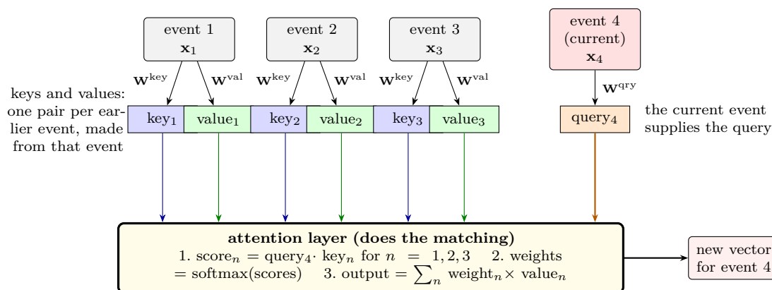
Figure 65: Attention on order-book events, for the newest event. Each earlier event is turned by learned matrices into a key (how it describes itself) and a value (what it passes on). The current event is turned into a query (what it is looking for). The attention layer scores the query against every key, converts the scores to weights, and sends the weighted average of the values back to the current event. In self-attention every event in the window takes its turn as the current one, each with its own query, against the keys and values of the events before it.
