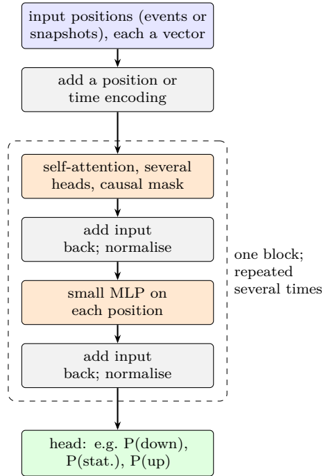
Figure 70: A Transformer. Each block mixes information across positions (self-attention) and then transforms each position on its own (MLP); blocks are stacked. Schematic.
