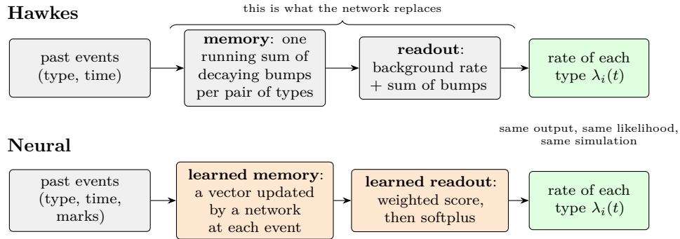
Figure 29: Parts of the Hawkes model replaced in a neural point process. Grey: kept from the Hawkes model. Orange: replaced by learned parts. Green: the output—a rate for each event type—is the same kind of object in both, so both are fitted by the same likelihood and simulated in the same way. Schematic.
