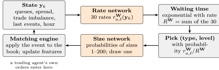
Figure 39: One step of the multidimensional deep queue-reactive simulator. Grey: the classical queue-reactive mechanism, unchanged (Figure 13). Orange: the two parts learned by networks. The paper reports 0.037 ms per generated event for the networks, excluding the matching engine.
