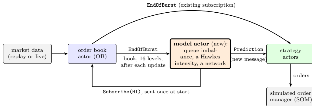
Figure 82: An order-book model added to KASPAR-HFT as an actor. It subscribes to the order book, receives the book after each burst of updates, and sends a prediction message to each strategy actor. Message names are those in the code; the model actor, the Prediction message and its handler in the strategy are new.
