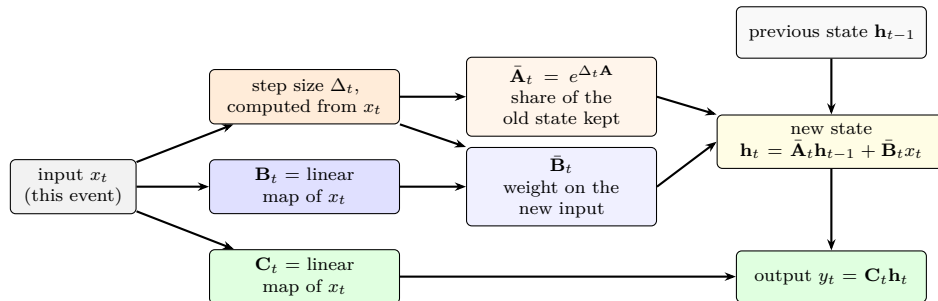
Figure 74: One step of Mamba’s selective state-space layer. The current input sets the step size \Delta_t and the matrices \mathbf{B}_t and \mathbf{C}_t ; the step size sets how much of the previous state survives. After Gu and Dao (2024).
