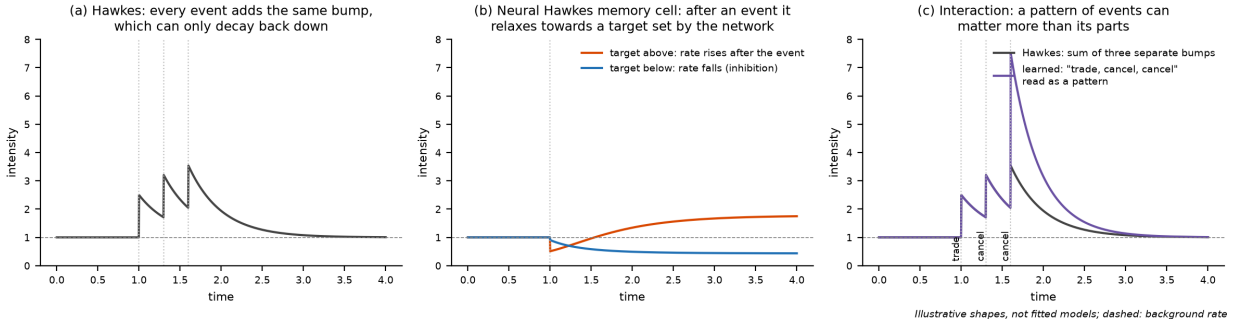
Figure 31: Intensity shapes that a fixed sum of bumps cannot produce. (a) A linear Hawkes intensity after three events: each adds the same bump, and between events the rate can only decay. (b) One memory cell of a continuous-time LSTM (Equation (40), Section 7.19.1): after an event the cell relaxes towards a target chosen by the network, so the rate can rise for a while after an event, or fall below the background rate (inhibition). (c) The same three events read as a pattern: a model that has learned that “trade, cancel, cancel” usually precedes a sweep raises the rate after the third event by more than the sum of three bumps. Hand-specified illustrative shapes, not fitted models.
