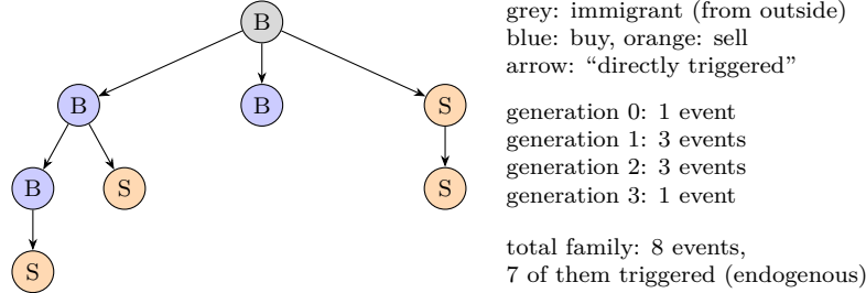
Figure 19: One family in a two-type Hawkes process. An immigrant buy triggers two buys and a sell (self- and cross-excitation), which trigger further events. The branching ratio is the average number of arrows leaving an event; for the process to be stable it must be below one, so that families die out. One illustrative family, drawn by hand; a branching ratio below one does not stop an individual family from being larger.
