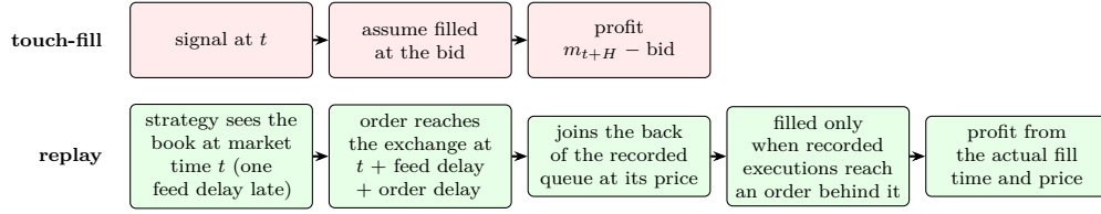
Figure 79: A touch-fill backtest and a queue-exact replay of the same passive order. The touch-fill backtest fills the order as soon as the signal fires; the replay sends it with its delays, places it in the recorded queue and fills it only when the recorded executions reach it.
