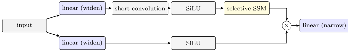
Figure 75: The Mamba block. The second branch gates the output of the selective state-space layer by multiplication. After Gu and Dao (2024) .
