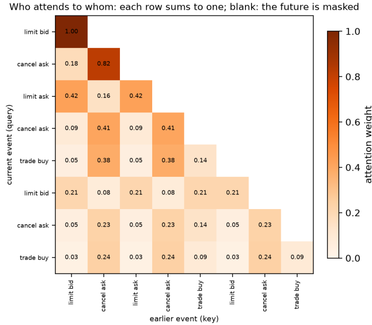
Figure 69: The attention weights of a whole sequence. Row n shows how event n divides its attention among events 1, \dots, n ; each row sums to one. Cells to the right of the diagonal are blank because an event may not attend to later events (masking, explained below). Hand-specified vectors, not a trained model.
