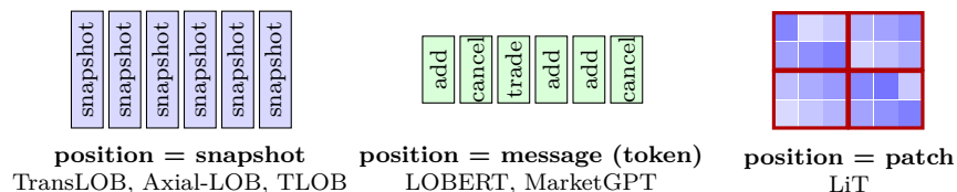
Figure 71: Three ways to cut order-book data into the positions a Transformer attends over. Only message positions are tokens drawn from a vocabulary. Schematic.
