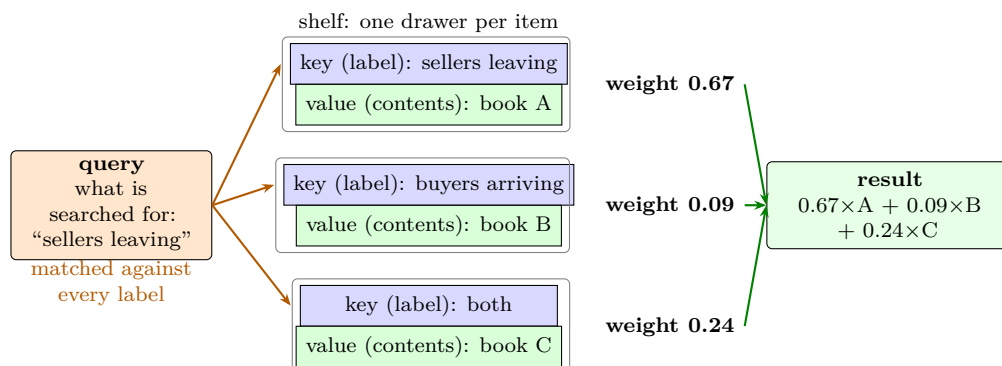
Figure 66: Attention as a library search. You bring a query; every drawer on the shelf carries a key (its label) and a value (its contents). The query is matched against every label, the matches become weights that sum to one, and you get back a mix of all the contents, mostly from the drawers that matched best. In the model, the query comes from the current event and each drawer is one earlier event (Figure 65). Numbers from the worked example below.
