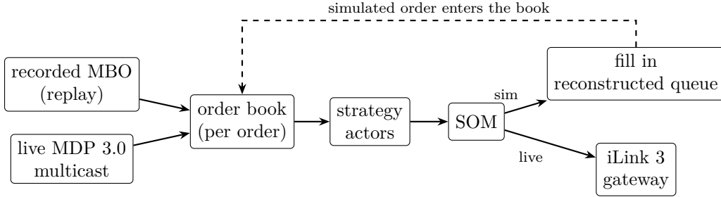
Figure 81: KASPAR-HFT data and order paths. Everything downstream of the market-data source is the same code in replay and live operation; the branch between simulated and live execution is a single decision in the simulated order manager.
