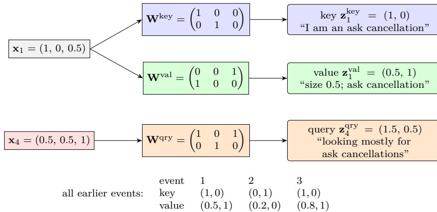
Figure 73: Step 2: each event’s embedding is multiplied by three learned matrices. The earlier events supply keys and values (top, for event 1; the table lists all three). The current event supplies the query (bottom). Example: \mathbf{W}^{\text{key}} \mathbf{x}_1 = (1 \cdot 1 + 0 \cdot 0 + 0 \cdot 0.5, 0 \cdot 1 + 1 \cdot 0 + 0 \cdot 0.5) = (1, 0) .
