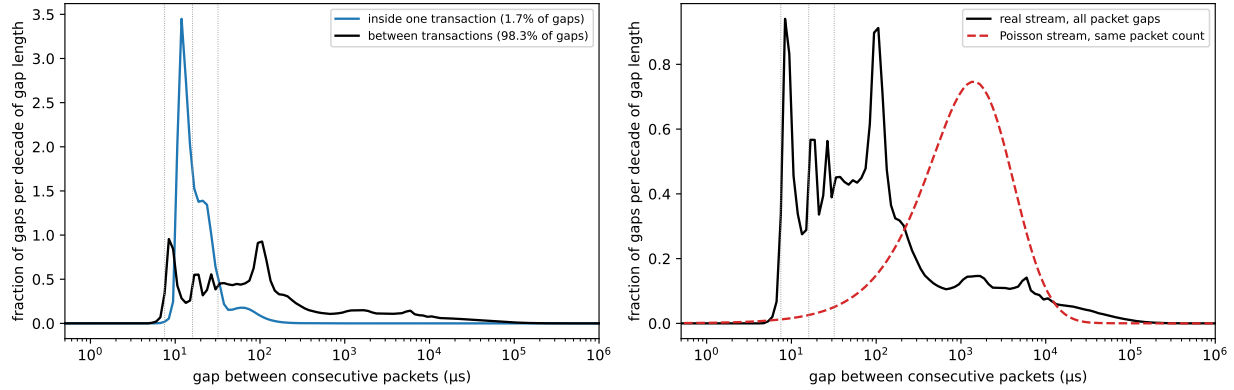
Figure 4. Packet interarrival gaps, pooled over the corpus. The gap axis is logarithmic and the vertical axis is the fraction of gaps per decade of gap length (twenty bins per factor of ten; the area under a curve between, say, 10 and 100 \mu\text{s} is the fraction of that curve's gaps in that range, and the total area is one). Dotted lines at 7.5, 16 and 32 \mu\text{s} . Left: gaps between two packets of the same transaction ( n = 5.6 \times 10^7 gaps) against gaps between packets of different transactions ( n = 3.24 \times 10^9 gaps). Each curve is normalised to its own total, so heights compare shapes, not counts (the blue gaps are 1.7% of all gaps, the black 98.3%). What it shows: the intra-transaction distribution is a single narrow peak at 12–16 \mu\text{s} with almost no mass below 10 \mu\text{s} and none below the floor — the pieces of one event are paced by the exchange at about 15 \mu\text{s} , slower than the closest that two packets of different events arrive, so the tightest gaps on the feed are never between pieces of the same event; the inter-transaction distribution has a sharp edge at the 7.5 \mu\text{s} floor, a broad plateau from the floor to about 30 \mu\text{s} , a second mode near 100 \mu\text{s} , and a long tail to seconds. Right: all packet gaps of the real stream (black; since 98.3% of gaps are between transactions this curve is the left panel's black curve with the blue one folded in) against the gaps of a Poisson stream with the same packet count over the same window (red, dashed), the distribution a receiver would face if the market's events were independent of one another at the observed rate. What it shows: the Poisson density is a single hump centred near 1 ms with negligible mass below 100 \mu\text{s} ; the real density puts a third of its mass below 32 \mu\text{s} , with the floor edge and the 100 \mu\text{s} mode absent from the null. The two curves are not two versions of the same shape: the real feed is not a Poisson stream, and the region in which it differs is exactly the region of gaps shorter than an HFT service time. What follows: the edge at 7.5 \mu\text{s} is a property of the gateway — no two packets of any origin are published closer than that — and it sets where a queue first forms; everything between the floor and 32 \mu\text{s} is gaps between different transactions, so the queueing regime of an HFT receiver is populated by distinct matching events arriving within one service time of each other, not by fragments of one event; and the whole of that region is absent from a Poisson stream at the same rate, which is why the uniform null in Table 2 has no tail below 32 \mu\text{s} . The 100 \mu\text{s} mode is the characteristic spacing of successive transactions within a burst, the time scale on which the self-excitation of Table 6 acts.
