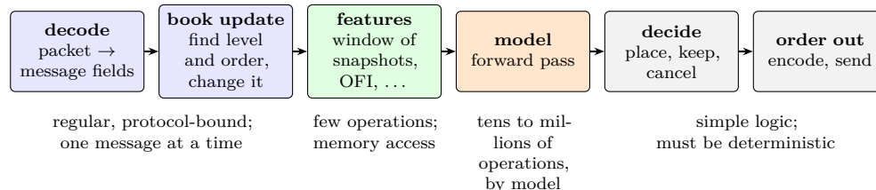
Figure 82: The per-event pipeline of a model-driven trading system. The model stage is the only one whose cost depends on the modeller’s choices. Schematic.
