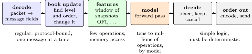
Figure 79: The per-event pipeline of a model-driven trading system. The model stage is the only one whose cost depends on the modeller’s choices. Schematic.
