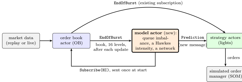
Figure 81: An order-book model added to Kaspar as an actor. It subscribes to the order book, receives the book after each burst of updates, and sends a prediction message to each strategy actor. Message names are those in the code; the model actor, the Prediction message and its handler in the strategy are new.
