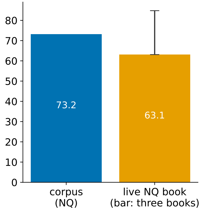
share of gaps &lt; mean/10 (%)
