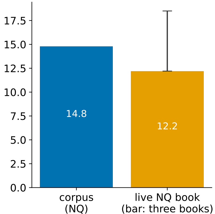
Fano collapse under shuffle (x)
