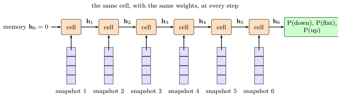
Figure 54: A recurrent network reads the snapshots in order. One cell, with one set of weights, updates a memory vector at each step; the memory after the last snapshot is used for the prediction. Schematic.
