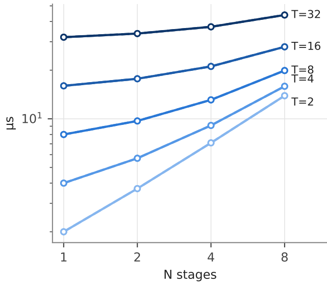
median latency vs N
