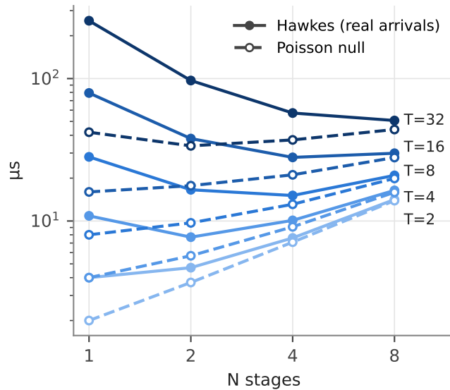
p99 latency vs N
