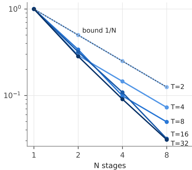
tail excess ratio \Delta(N)/\Delta(1)
