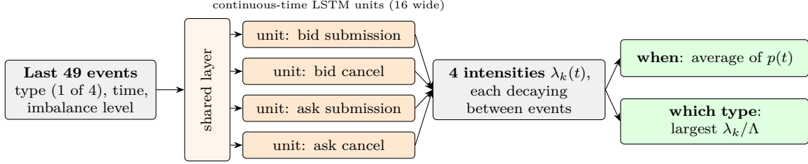
Figure 41: The state-dependent parallel neural Hawkes process of Shi and Cartlidge (2022) , as used for prediction. Grey: inputs and the Hawkes-type intensities. Orange: the learned parts. Green: the two predictions. Schematic; the learned matrix of state transitions is not drawn.
