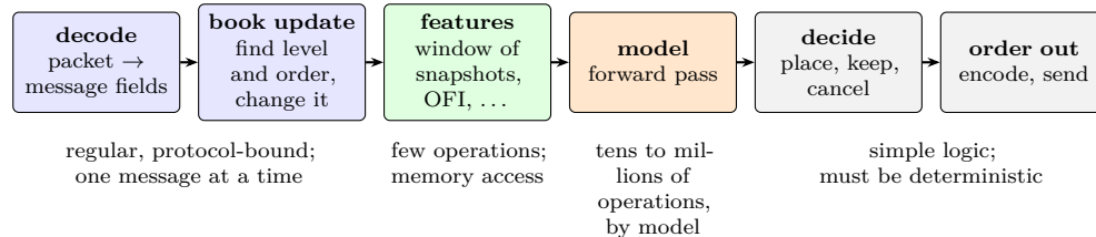
Figure 88: The per-event pipeline of a model-driven trading system. The model stage is the only one whose cost depends on the modeller’s choices. Schematic.
