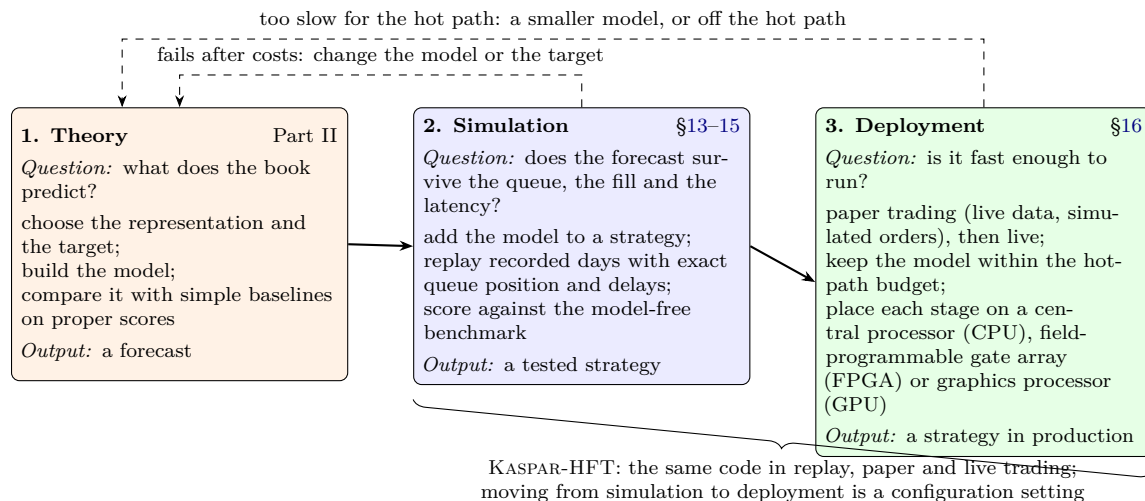
Figure 1: The path from theory to production that the survey follows. Each stage asks its own question and passes on its output only if the answer is yes; a strategy that fails in simulation, or a model too slow for the hot path, goes back to the first stage.
