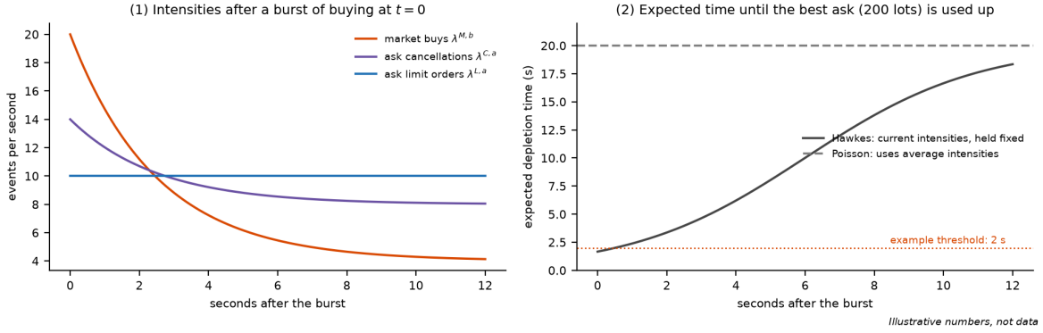
Figure 34: Depletion time after a burst. (1) Intensities at the best ask after a burst of buying at time zero, decaying back to normal. (2) Expected time until the 200-lot best ask is used up, computed from the current intensities held fixed (solid), against the Poisson answer from average intensities (dashed). For a few seconds after the burst the Hawkes estimate is a fraction of the Poisson one; a trader whose cancellation takes longer than the dotted threshold is at risk in that window. Illustrative numbers, not data.
