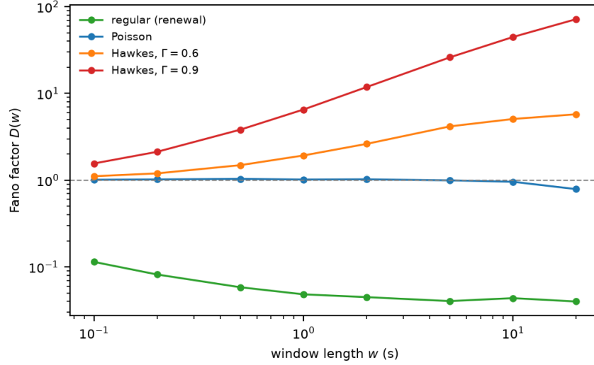
Figure 23: The Fano factor D(w) against the window length w on logarithmic axes, for the four processes of Figure 21 simulated over 3,000 seconds. Regular renewal process: below one, settling near 0.04. Poisson: flat at one. Hawkes with \Gamma = 0.6 : rising, then levelling off as the window becomes long compared with the one-second kernel. Hawkes with \Gamma = 0.9 : a steeper rise, with a slope of about 0.7 over windows from 0.1 to 2 seconds, which the Hurst formula would read as \mathcal{H} \approx 0.84 ; with an exponential kernel this growth also levels off eventually, at D = 1/(1 - \Gamma)^2 = 100 . Redrawn after Maciejewski (2026b) ; stylised simulation.
