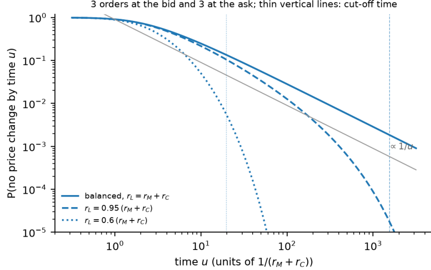
Figure 9: Cont–de Larrard model: probability that the price has not changed by time u , starting from three orders at each best quote, computed from the closed-form expression, on logarithmic axes. Time is in units of the mean time between departures from a queue. Balanced rates (solid) give a 1/u tail and an infinite mean waiting time; with inflow below outflow (dashed, dotted) the curve breaks away exponentially, later the closer the rates are to balance. Stylised rates.
