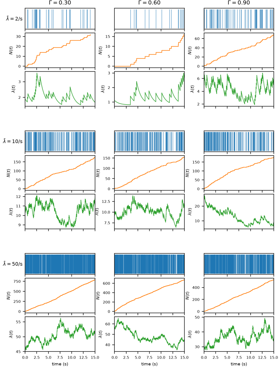
Figure 20: Simulated exponential-kernel Hawkes processes. Each cell stacks the event raster (top), the cumulative count N(t) (middle) and the intensity \lambda(t) (bottom). Rows: long-run rate \bar{\lambda} \in \{2, 10, 50\} events per second. Columns: branching ratio \Gamma \in \{0.30, 0.60, 0.90\} . Fifteen seconds, decay rate \omega = 1/s . The time scale is chosen for legibility; the kernel fitted on CME data decays about four orders of magnitude faster. Each process is simulated by thinning after a burn-in period, so it starts in its long-run regime. Redrawn after Maciejewski (2026b) ; stylised simulation.
