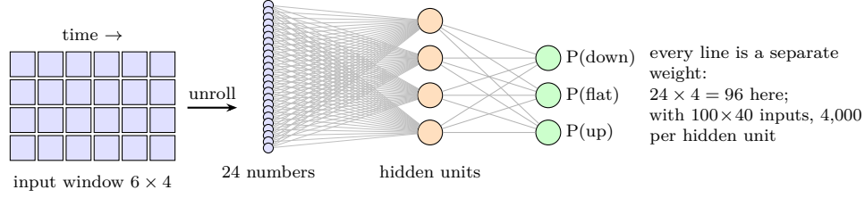
Figure 55: A fully connected network on a window of the book. The window is unrolled into a list, and every input is connected to every hidden unit by its own weight. Schematic.
