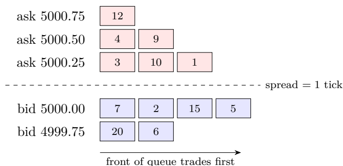
Figure 2: A small book. Each box is one waiting order and the number is its size in lots. Orders at the same price form a first-in-first-out queue, front on the left. The best bid is 5000.00 with 7 + 2 + 15 + 5 = 29 lots; the best ask is 5000.25 with 14 lots; the spread is one tick of 0.25.
