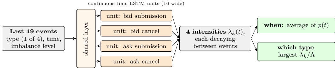
Figure 41: The state-dependent parallel neural Hawkes process of Shi and Cartlidge (2022), as used for prediction. Grey: inputs and the Hawkes-type intensities. Orange: the learned parts. Green: the two predictions. Schematic; the learned matrix of state transitions is not drawn.
