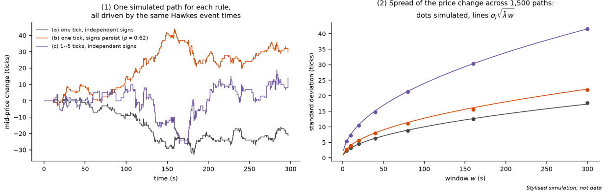
Figure 24: Compound Hawkes prices. Event times come from a Hawkes process with an exponential kernel, background rate 0.5 per second and branching ratio 0.5, so \bar{\lambda} = 1 move per second. (a) Moves of one tick with independent directions; (b) moves of one tick that repeat the previous direction with probability p = 0.62 ; (c) moves of 1 to 5 ticks with independent directions. (1) One path for each rule. (2) Standard deviation of the price change over a window, across 1,500 simulated paths (dots), against \sigma_J \sqrt{\lambda w} (lines), with \sigma_J^2 = 1 , p/(1-p) and the mean squared move size respectively; the simulated values lie within about 7% of the lines. Stylised simulation; not data.
