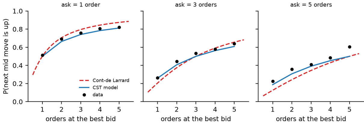
Figure 11: Probability that the next mid move is up for three sizes of the ask queue: the Cont-de Larrard formula (2/\pi) \arctan(v^b/v^a) (dashed), the Cont-Stoikov-Talreja model (solid) and the empirical frequencies (dots) of Table 11. The arctan formula uses no fitted parameters.
