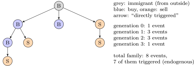
Figure 19: One family in a two-type Hawkes process. An immigrant buy triggers two buys and a sell (self- and cross-excitation), which trigger further events. The branching ratio is the average number of arrows leaving an event; for the process to be stable it must be below one, so that families die out. One illustrative family, drawn by hand; a branching ratio below one does not stop an individual family from being larger.
