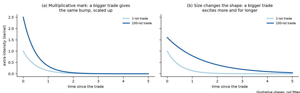
Figure 26: Two ways a trade’s size can change its effect on later events. (a) Multiplicative: the bump keeps its shape and is scaled up. (b) Non-separable: a larger trade’s bump is higher and decays more slowly. On Bund and DAX futures the data favour (b) (Rambaldi et al., 2017). Illustrative shapes, not fitted.
