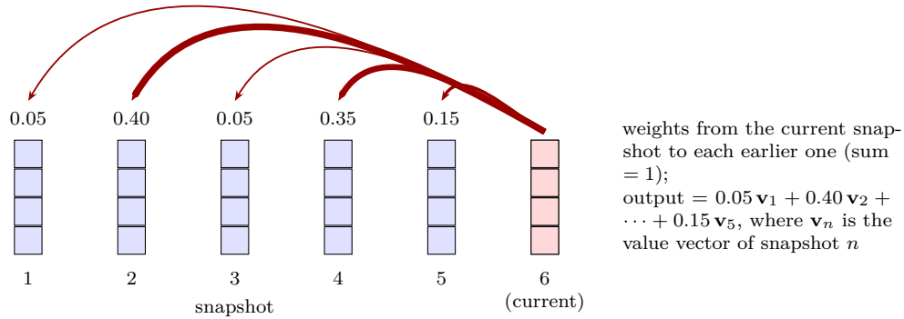
Figure 59: Attention: the current snapshot weights every earlier snapshot by how well they match, and takes the weighted average of their values. Line width shows the weight; numbers are illustrative. Schematic.
