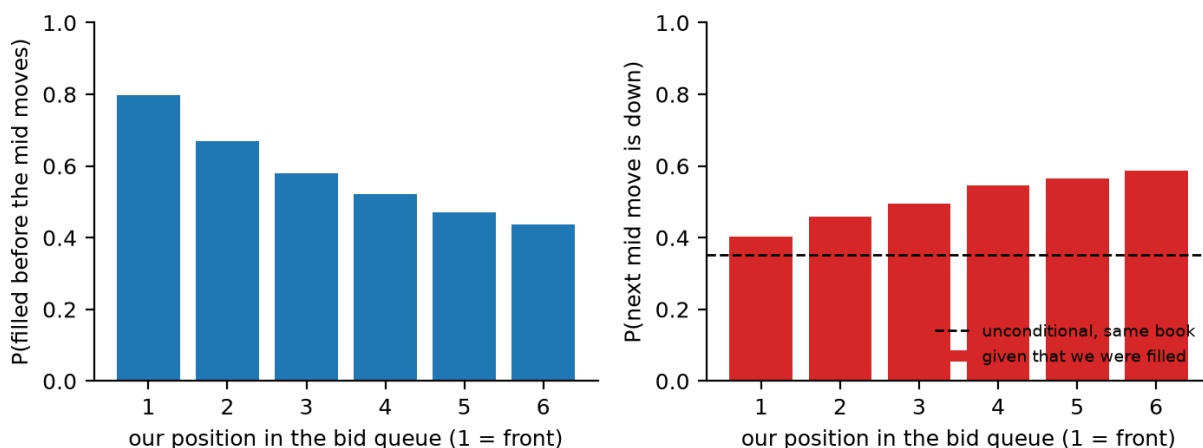
Figure 13: Adverse selection by queue position, Cont–Stoikov–Talreja model with the rates of Table 10: six orders at the best bid (ours at the position shown), three at the ask. Left: probability that our order is filled before the mid moves. Right: probability that the next mid move is down, among the paths on which our order was filled (bars), against the probability of a down move from the same book with no conditioning (dashed). Stylised simulation for illustration; not data.
