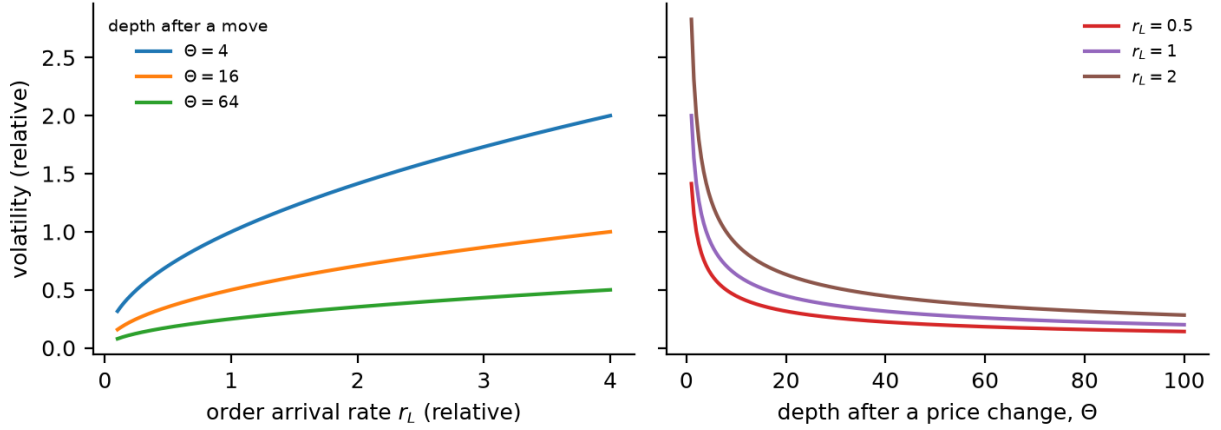
Figure 12: Cont-de Larrard model: volatility \propto \delta\sqrt{r_L/\Theta} , in relative units, against the order arrival rate for three depths (left) and against the depth after a price change for three arrival rates (right). Busier markets are more volatile; markets that refill deeply after each move are calmer.
