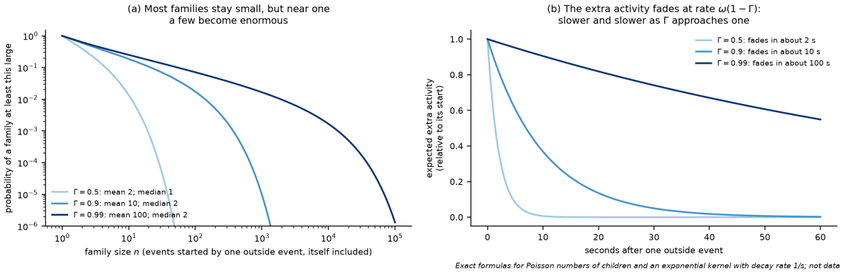
Figure 25: Near-criticality. (a) Probability that the family of events started by one outside event has at least n events, for branching ratios 0.5, 0.9 and 0.99 (log scales). The mean family size is 1/(1 - \Gamma) , but the median stays at one or two; near one the mean is carried by rare, very large families. (b) Expected extra activity after one outside event, for an exponential kernel with decay rate one per second: it fades at rate \omega(1 - \Gamma) , so the time to calm down is 1/(\omega(1 - \Gamma)) . Exact formulas, not data.
