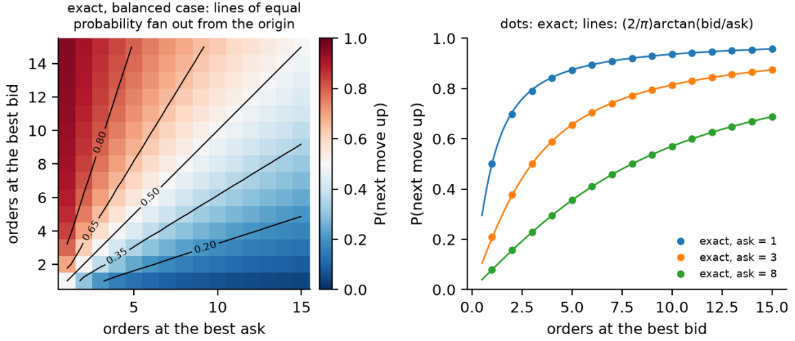
Figure 10: Cont-de Larrard model, balanced case: probability that the next mid move is up. Left: the exact expression of the paper’s Proposition 2 over a grid of queue sizes; the contours of equal probability are nearly straight lines through the origin, so the probability depends mainly on the ratio of bid to ask. Right: the exact values (dots) against the simple form (2/\pi) \arctan(v^b/v^a) (lines), which is already very close for small queues. Neither depends on any rate: in the balanced case only the queue sizes matter.
