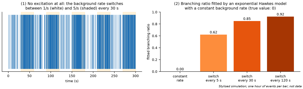
Figure 33: A branching ratio from no excitation. (1) A stream of events with no self-excitation; only the background rate changes, between 1 and 5 per second. (2) The branching ratio estimated by maximum likelihood with an exponential Hawkes model that assumes a constant background rate, for one hour of events: zero when the rate is truly constant, 0.62 to 0.92 when it switches every 5, 30 or 120 seconds. Stylised simulation; not data.
