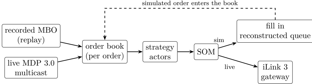
Figure 86: KASPAR-HFT data and order paths. Everything downstream of the market-data source is the same code in replay and live operation; the branch between simulated and live execution is a single decision in the simulated order manager.
