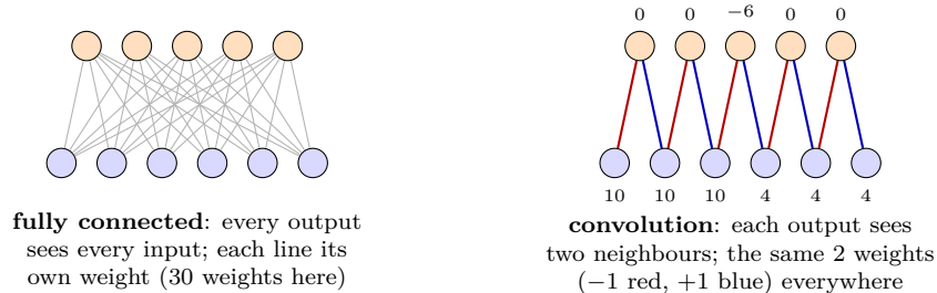
Figure 62: A fully connected layer and a convolution on the same six inputs, the size of the best bid over six events. The convolution with weights (-1, +1) detects the drop from 10 to 4 wherever it occurs. Illustrative numbers. Schematic.
