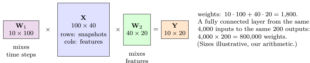
Figure 58: A bilinear layer: the window matrix is multiplied on the left by a matrix that mixes time steps and on the right by a matrix that mixes features. Schematic.
