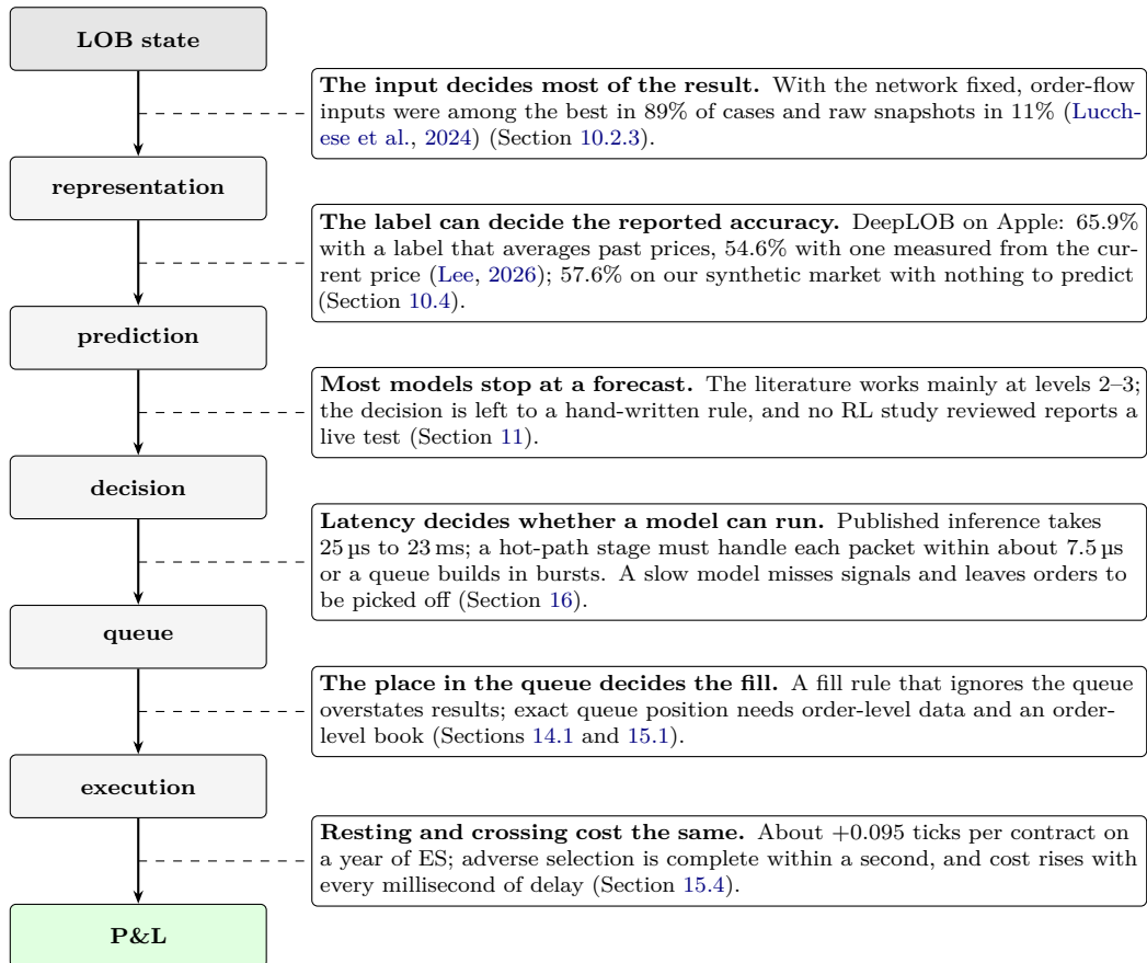
Figure 90: The chain from order book to profit, with what the survey found at each link and where. Figures are those quoted in the sections named, with their sources there.
