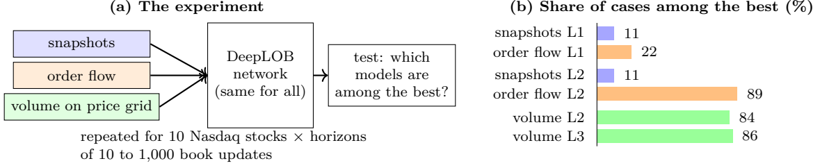
Figure 53: The input experiment of Lucchese et al. (2024) . (a) Only the input changes; the network is fixed. “Among the best”: not shown to be worse than the best model by a model confidence set test at the 1% level. (b) Share of (stock, horizon) cases in which each input was among the best, stock-specific models (their Table 5). L1, L2, L3: the paper’s labels for variants of each input. Several inputs can be among the best in the same case, so the shares do not sum to 100%.
