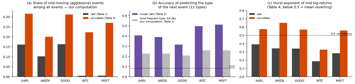
Figure 44: Results of Lalor and Swishchuk (2025), re-plotted; not our data. (a) Share of the six mid-moving event types among all events, real and simulated, which we computed from the paper’s event counts. (b) Test accuracy of predicting the next event’s type, beside the share of the most frequent type over the whole day (our computation; a rough reference, not the paper’s baseline). (c) Hurst exponent of mid log-returns, real and simulated.
