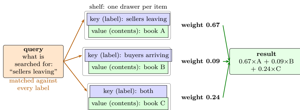
Figure 67: Attention as a library search. You bring a query; every drawer on the shelf carries a key (its label) and a value (its contents). The query is matched against every label, the matches become weights that sum to one, and you get back a mix of all the contents, mostly from the drawers that matched best. In the model, the query comes from the current event and each drawer is one earlier event (Figure 66). Numbers from the worked example below.
