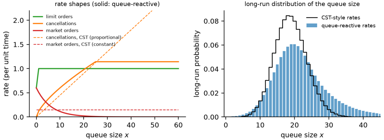
Figure 15: Queue-reactive rates and the long-run distribution of the queue size. Left: stylised rate functions with the shapes reported by Huang et al. (2015)—roughly constant arrivals, cancellations that rise and then flatten, market orders that fall off as the queue grows (solid)—against Cont–Stoikov–Talreja style rates with proportional cancellation and constant market orders (dashed). Right: the long-run distributions implied by each, from the balance formula. Because cancellations stop growing for long queues, long queues are much more likely under the queue-reactive shapes. Stylised rates, not fitted values.
