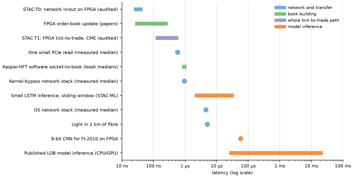
Figure 89: Latency figures quoted in this section, on one logarithmic axis. Bars are ranges, dots single figures. Sources: STAC public summaries (audited), the FPGA book-building papers, the measured server latency budget (Zilberman et al., 2017), KASPAR-HFT’s socket-to-book book medians (Maciejewski, 2026a), and Table 62. The figures come from different machines, conditions and years and show orders of magnitude, not a single system.
