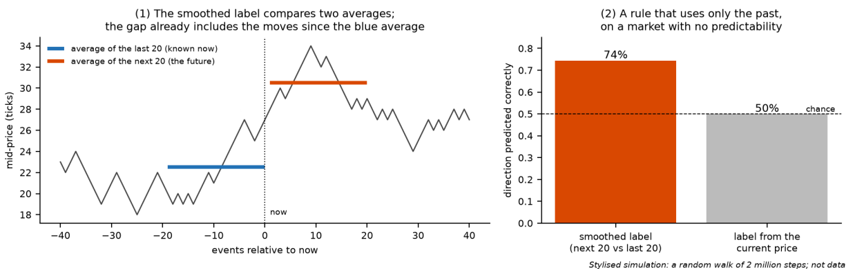
Figure 61: Why a smoothed label inflates accuracy. (1) The label compares the average of the next 20 mid-prices with the average of the last 20; at “now” the price is already above its recent average, so part of the gap is already known. (2) On a pure random walk, where nothing can be predicted, a rule using only the past gets the direction of the smoothed label right 74% of the time, and the direction of a label measured from the current price 50% of the time. Stylised simulation, not data.
