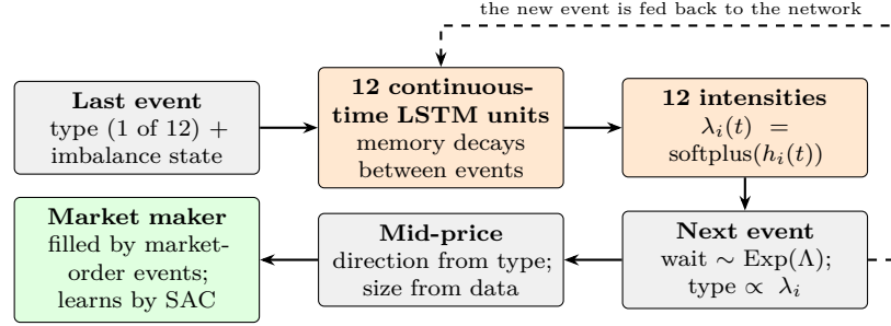
Figure 43: The pipeline of Lalor and Swishchuk (2025). Grey: the Hawkes skeleton (event types, thinning, mid moves by event type). Orange: the learned part, which replaces the sum of exponential kernels. Green: the trading agent. The simulated event stream is generated first; the agent’s quotes are filled by its market-order events but are not part of it.
