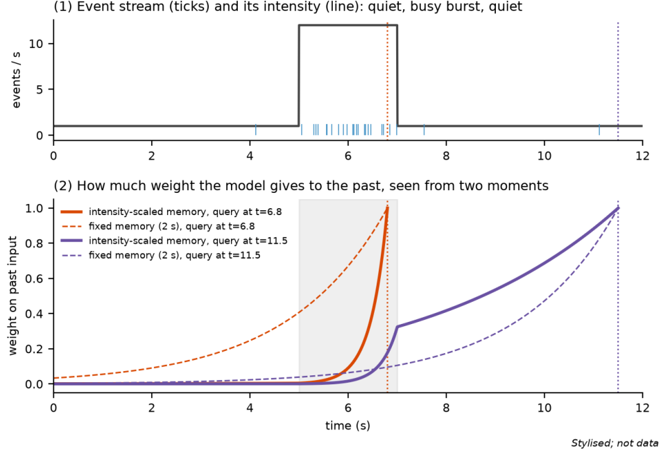
Figure 47: Memory scaled by event intensity versus fixed memory. (1) An event stream with a two-second burst (shaded below). (2) Weight that the model’s state gives to past inputs, seen from inside the burst ( t = 6.8\text{s} ) and from a quiet period ( t = 11.5\text{s} ). Solid: memory fades by a fixed factor per expected event, e^{-\frac{1}{4} \times (\text{expected events since then})} . Dashed: memory fades with a fixed time constant of 2 s. Stylised; not data. This is the proposed design, not a published model.
