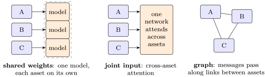
Figure 83: Three ways deep models connect several assets. Schematic.
