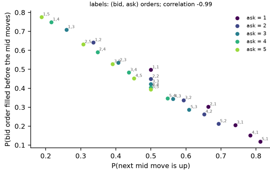
Figure 8: For each combination of queue sizes (labels: orders at the bid, orders at the ask), the model's probability that the next move is up (horizontal) against the probability that an order at the back of the bid is filled before the mid moves (vertical); values from Tables 11 and 12. High fill probability comes with a likely down move: the fills a resting bid gets are disproportionately the bad ones.
