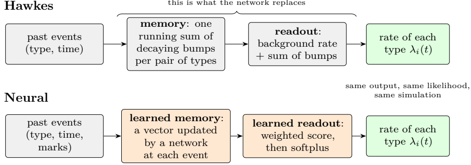
Figure 29: What a neural point process replaces. Grey: kept from the Hawkes model. Orange: replaced by learned parts. Green: the output—a rate for each event type—is the same kind of object in both, so both are fitted by the same likelihood and simulated in the same way. Schematic.
