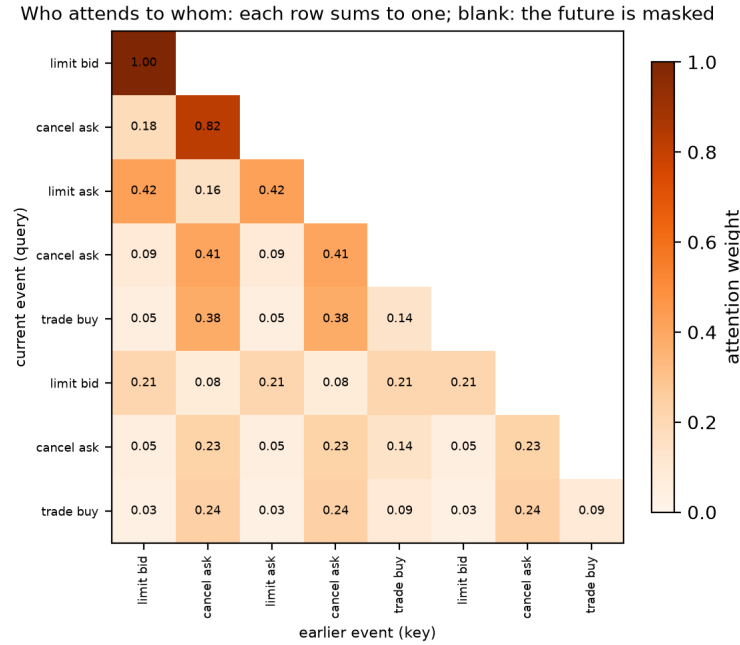
Figure 70: The attention weights of a whole sequence. Row n shows how event n divides its attention among events 1, \dots, n ; each row sums to one. Cells to the right of the diagonal are blank because an event may not attend to later events (masking, explained below). Hand-specified vectors, not a trained model.
