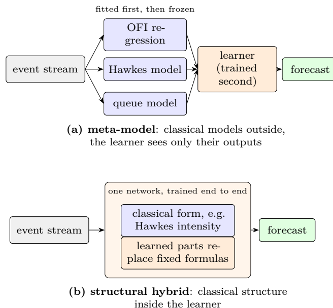
Figure 38: The difference between a meta-model and a structural hybrid. (a) Classical models are fitted separately and frozen; a second-stage learner combines their outputs. (b) A single network reads the events and has the form of a classical model, with some of its fixed formulas replaced by learned functions; everything is trained together. Schematic.
