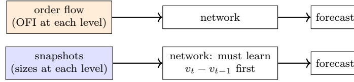
Figure 54: Our interpretation of Figure 53. Given order flow, the network receives OFI ready-made. Given snapshots, it must first learn to subtract consecutive sizes from the training data. Schematic.
