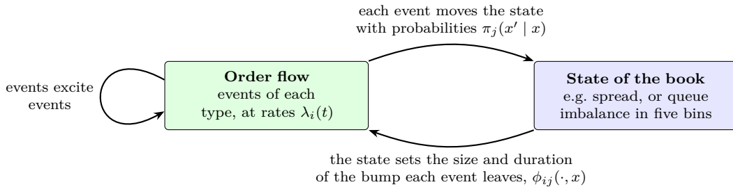
Figure 27: The feedback loop of a state-dependent Hawkes process ( Morariu-Patrichi and Pakkanen, 2022 ). An ordinary Hawkes process has only the loop on the left; a queue-reactive model has a state, but no excitation between events. Schematic.
