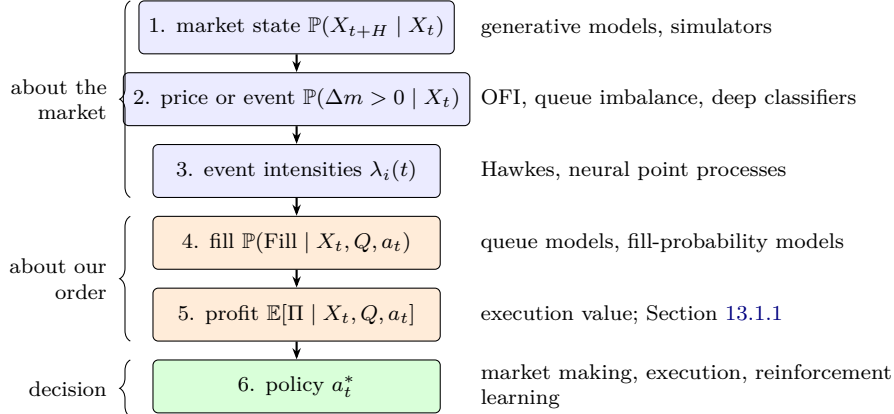
Figure 4: The hierarchy of prediction objectives, with the model families that work at each level. Our synthesis.
