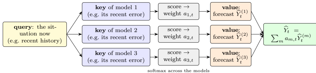
Figure 37: Attention used to combine forecasts. The query describes the current situation, each model has a key, the match between them sets the model’s weight, and the combined forecast is the weighted average of the models’ forecasts (the values). Schematic.
