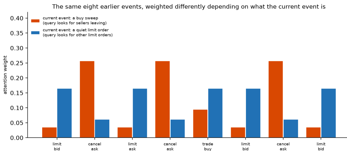
Figure 69: The same eight earlier order-book events, weighted by two different queries. Orange: the current event is a buy sweep, whose query looks for sellers leaving; the ask cancellations receive most of the weight. Blue: the current event is a quiet limit order, whose query looks for other limit orders. Hand-specified vectors, not a trained model.
