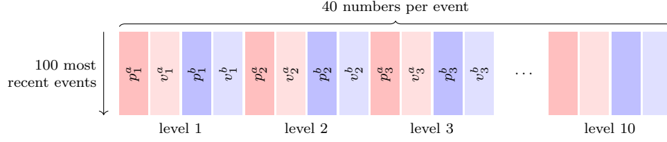
Figure 63: The input of DeepLOB: the last 100 snapshots of the book, each laid out as price and size, ask then bid, level by level. Red: ask side; blue: bid side. Schematic.
