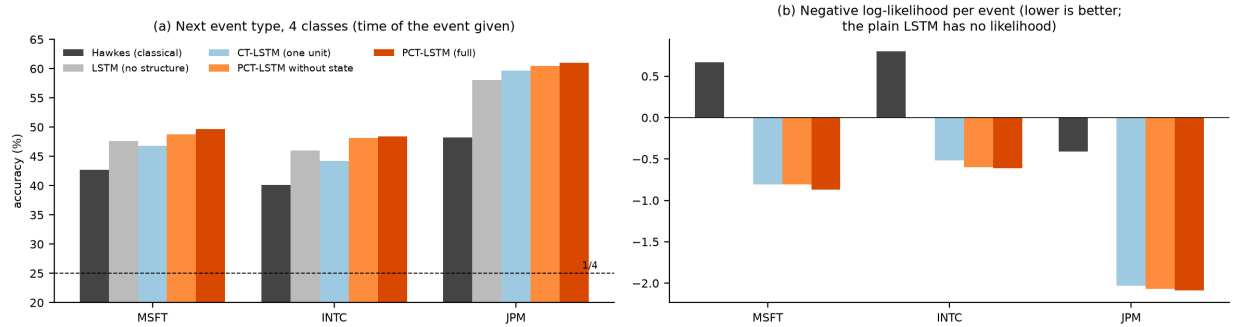
Figure 42: Results reported by Shi and Cartlidge (2022), Table 1, re-plotted; not our data. (a) Accuracy of predicting the type of the next event, with the time of the event given; dashed line: guessing among four types. (b) Negative log-likelihood per event; the plain LSTM has no likelihood.
