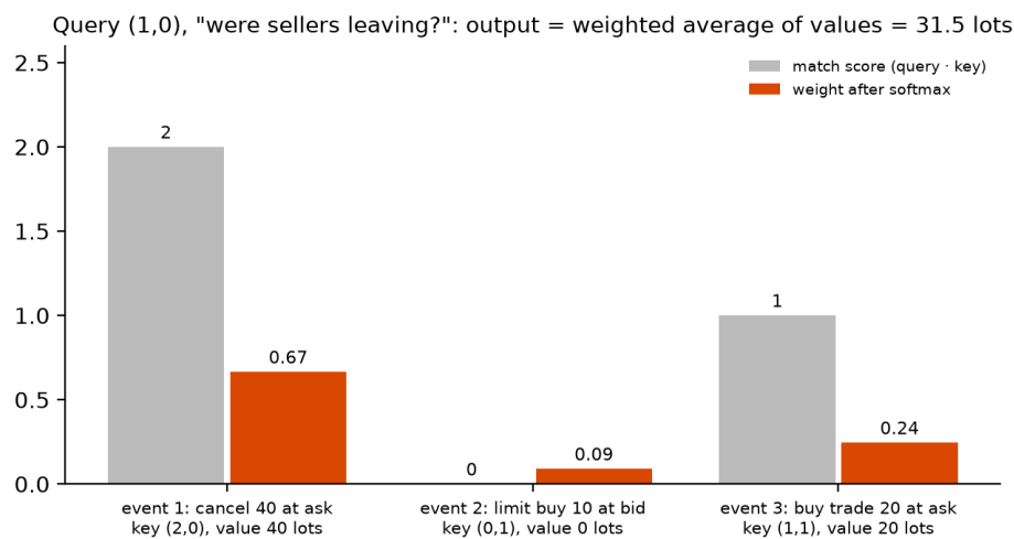
Figure 68: The worked example above. Grey: the score of each earlier event, the match of its key with the query (1,0), "were sellers leaving?". Orange: the weights the softmax turns the scores into. The output is the weighted average of the values, 31.5 lots. Hand-made numbers.
