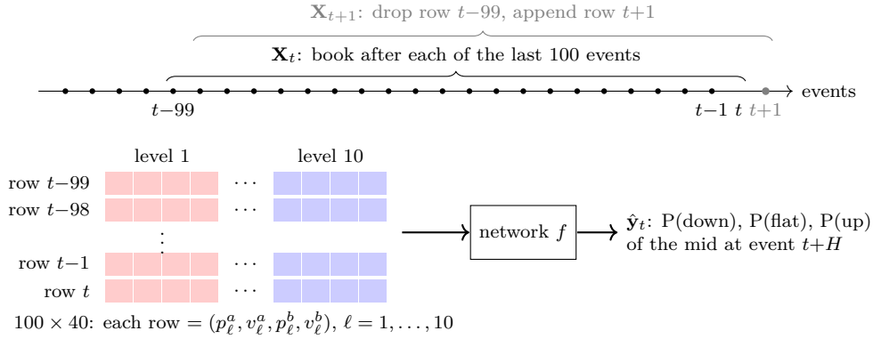
Figure 51: How a snapshot model looks back. After each event the first ten levels of the book are written as one row of 40 numbers. The input \mathbf{X}_t stacks the rows for the last 100 events. One forecast is made per event; at the next event the window moves by one row. Schematic.
