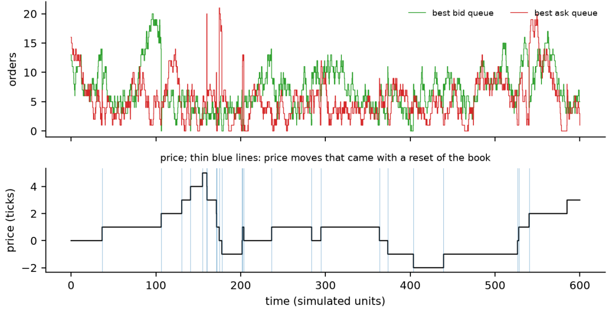
Figure 16: A run of a queue-reactive simulator with two levels per side, rate functions of the shapes in Figure 15 scaled to short queues, \pi_{\text{move}} = 0.7 and \pi_{\text{reinit}} = 0.85 . Top: sizes of the best bid and best ask queues. Bottom: the price, in ticks; thin vertical lines mark price moves that came with a reset of the book. Stylised simulation for illustration; not data.
