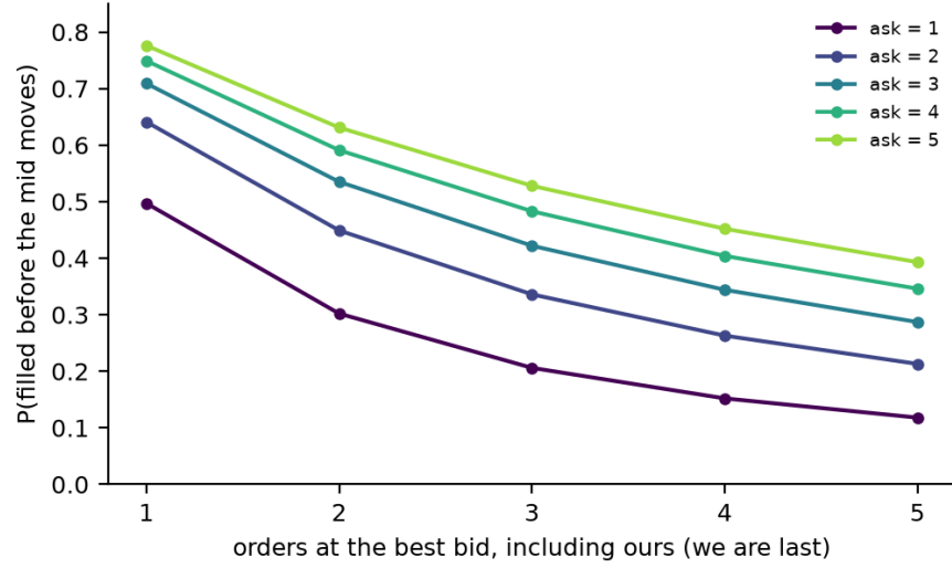
Figure 7: Probability that an order at the back of the best bid is filled before the mid moves, against the length of the bid queue (our order included and last), one curve per size of the best-ask queue; model values from Table 12. Every order ahead of ours lowers the chance; a long ask queue raises it, because it makes the price less likely to move up and away before we are reached.
