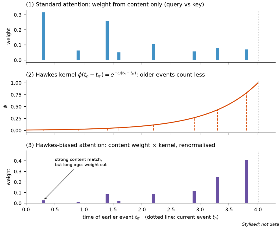
Figure 46: Hawkes-biased attention for one current event (dotted line) and eight earlier events. (1) Weights from content alone. (2) Exponential kernel, \omega = 1.2 per second. (3) Weights after the log kernel is added to the scores: each content weight is multiplied by the kernel and the result is renormalised to sum to one. Stylised; the content scores are invented for illustration.
