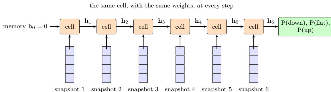
Figure 57: A recurrent network reads the snapshots in order. One cell, with one set of weights, updates a memory vector at each step; the memory after the last snapshot is used for the prediction. Schematic.
