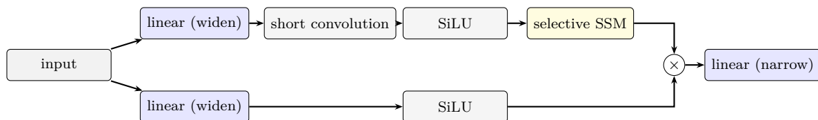
Figure 80: The Mamba block. The second branch gates the output of the selective state-space layer by multiplication. After Gu and Dao (2024).
