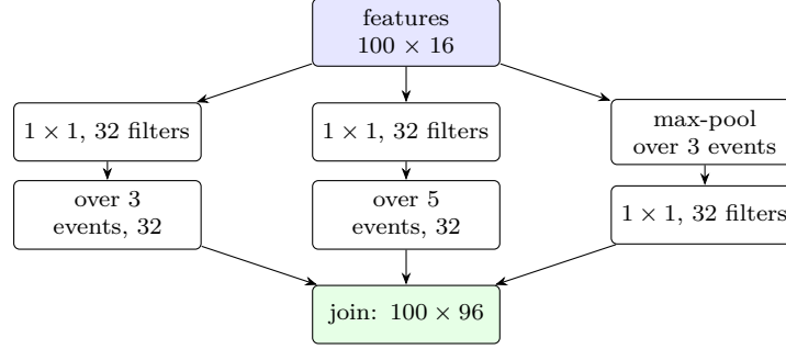
Figure 65: The Inception module of DeepLOB: three branches look at the same features over different time scales, and their outputs are joined. After Zhang et al. (2019a).
