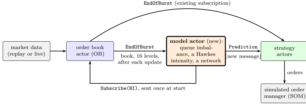
Figure 87: An order-book model added to KASPAR-HFT as an actor. It subscribes to the order book, receives the book after each burst of updates, and sends a prediction message to each strategy actor. Message names are those in the code; the model actor, the Prediction message and its handler in the strategy are new.
