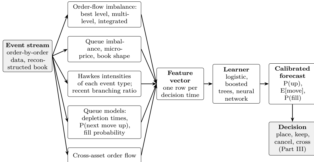
Figure 35: A meta-model. Classical models of the book (left) each turn the event stream into a few interpretable numbers; a learner (right) combines them into a calibrated forecast for the execution decision. The classical models are fitted first and kept fixed while the learner is trained on their out-of-sample outputs (Section 8.7).
