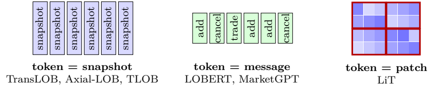
Figure 72: Three ways to cut order-book data into the tokens a Transformer attends over. Schematic.
