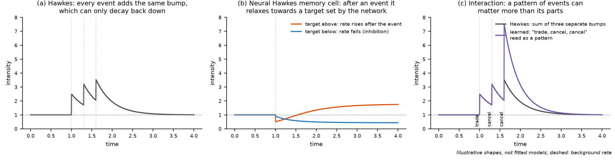
Figure 31: What a fixed sum of bumps cannot draw. (a) A linear Hawkes intensity after three events: each adds the same bump, and between events the rate can only decay. (b) One memory cell of a continuous-time LSTM (Equation (40), Section 7.19.1): after an event the cell relaxes towards a target chosen by the network, so the rate can rise for a while after an event, or fall below the background rate (inhibition). (c) The same three events read as a pattern: a model that has learned that “trade, cancel, cancel” usually precedes a sweep raises the rate after the third event by more than the sum of three bumps. Hand-specified illustrative shapes, not fitted models.
