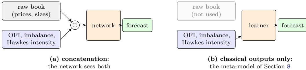
Figure 45: Concatenation. (a) The classical outputs ( \oplus : placed side by side) are extra inputs next to the raw book. (b) Remove the raw book and the same design is a meta-model. Comparing (a) with a network on the raw book alone is the ablation of Example 9.1. Schematic.
