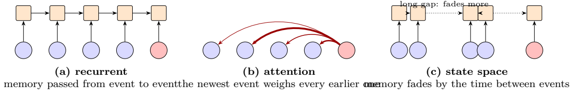
Figure 32: Three ways a neural point process builds its memory of the past. Blue: earlier events; red: the newest event; orange: memory. (a) A recurrent network (RMTPP, neural Hawkes) updates its memory event by event. (b) An attention model (Transformer Hawkes, self-attentive Hawkes) compares the newest event with every earlier event and weights them, the thickness of the arrows. (c) A state-space model (Mamba Hawkes) updates its memory event by event, letting it fade more across a longer gap in time. Schematic.
