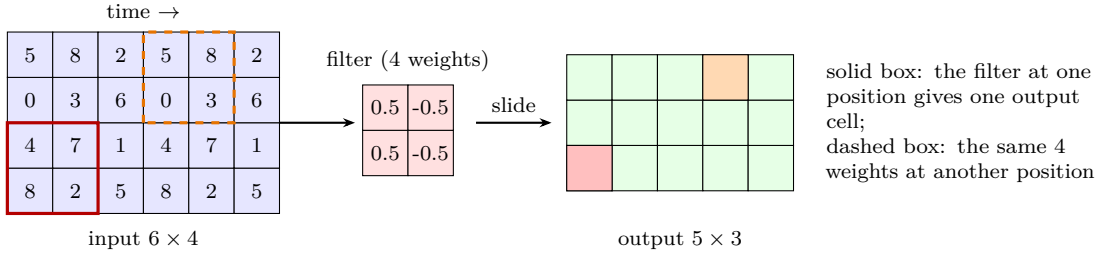
Figure 56: A convolution. One 2 \times 2 filter of weights is applied at every position of the input; each position gives one number of the output. Numbers are illustrative. Schematic.
