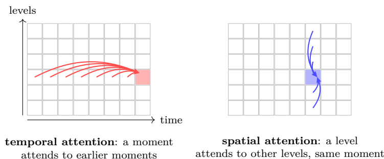
Figure 77: Attention along two axes of a window of snapshots. Temporal attention (left) lets the current moment weight earlier ones; spatial attention (right) lets each price level weight the other levels at the same moment. Schematic.
