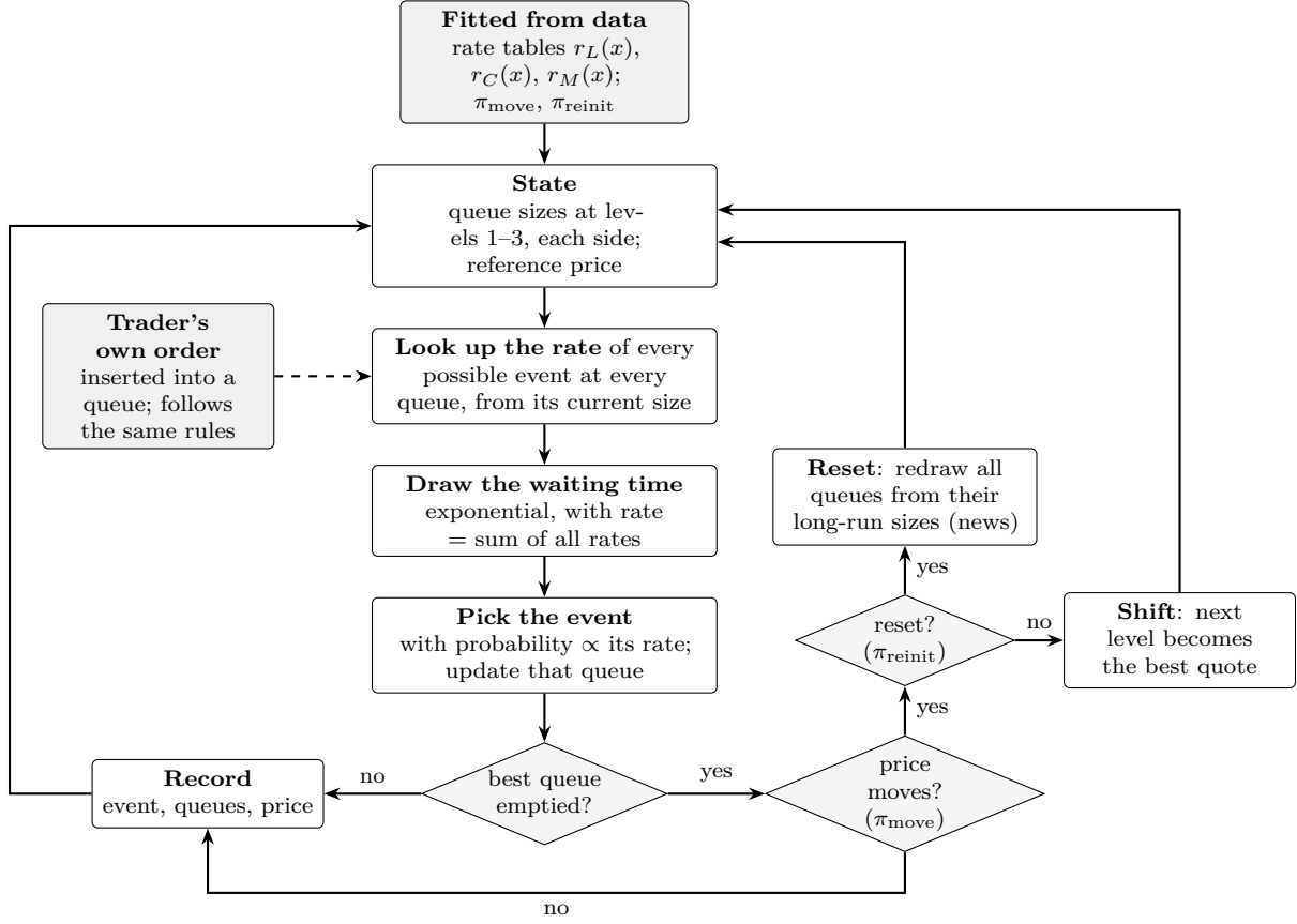
Figure 14: One step of the queue-reactive simulator. The fitted rate tables are the only input from data. At every step the rates are looked up from the current queue sizes, so the simulated book reacts to its own history and to any order the trader inserts. Price moves come from emptied best queues; most of them, in the calibration of Huang et al. (2015) , come with a reset of the whole book that stands for news.
