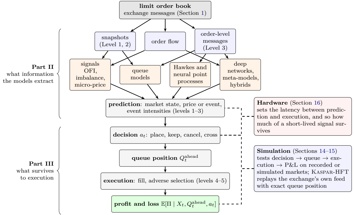
Figure 3: A map of the survey. The limit order book reaches models through one of three representations; the models produce predictions; a decision turns a prediction into an order, which takes a place in a queue and may be filled. Part II covers the upper half, Part III the lower half, with simulation and hardware attached where they act.
