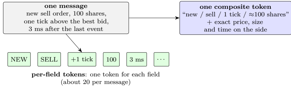
Figure 78: Two ways of tokenising the same message. Field-level schemes (Nagy et al., 2023) emit one token per field; event-level schemes (Linna et al., 2025) map the whole event to a single token from a vocabulary of binned combinations, and may pass the exact values alongside. Schematic.
