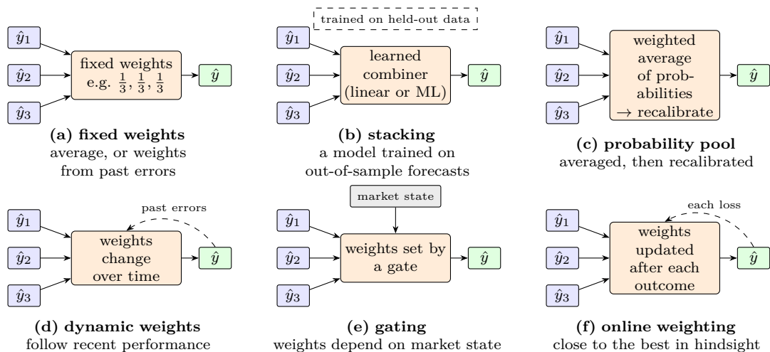
Figure 36: Six ways to combine the forecasts of several models into one. Schematic.
