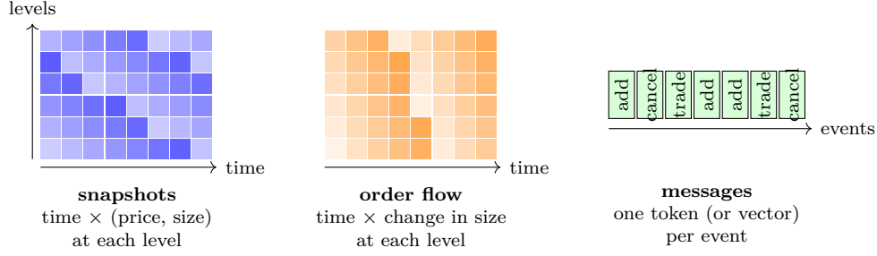
Figure 50: Three ways of presenting the book to a network: a window of snapshots of the first levels; the same window transformed into order flow (changes in size at each level); or the sequence of individual messages. Schematic.
