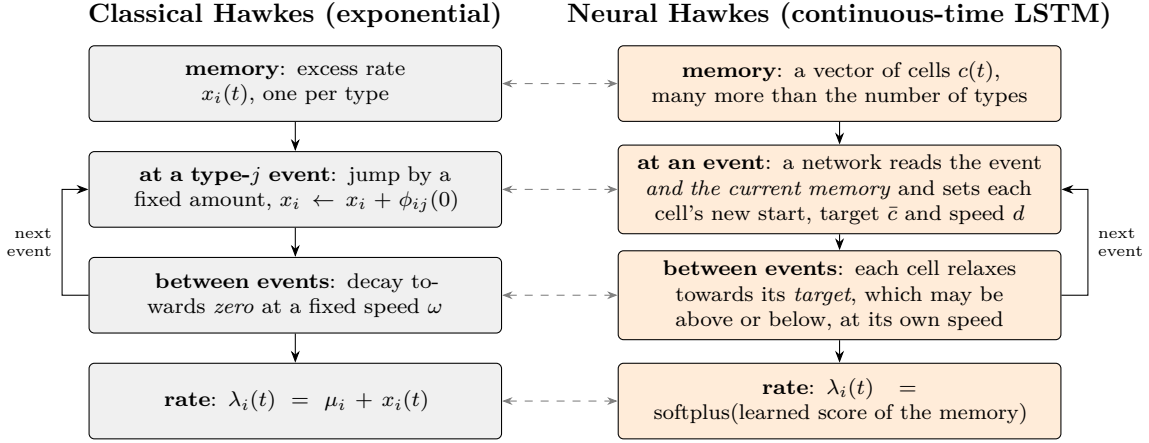
Figure 30: One step of the classical exponential Hawkes model (left) and of the neural Hawkes process (Mei and Eisner, 2017) (right). Dashed arrows join corresponding parts. The classical model has the same shape as the neural one with the jump fixed by the kernel, the target fixed at zero and the speed fixed at \omega ; the neural model computes all three from the history at every event. Schematic.
