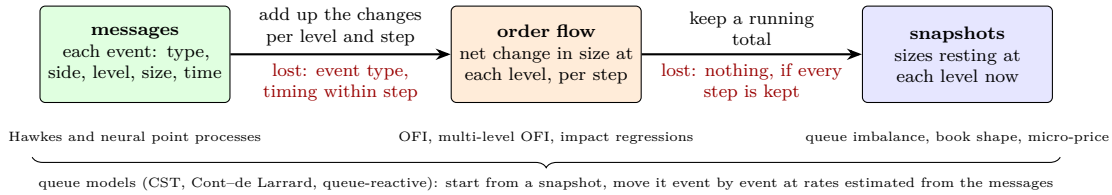
Figure 52: The three inputs of Figure 50 are one event stream summarised to different degrees. Summing messages into order flow loses the event types and their timing, which cannot be recovered. Below each input: the classical models of Sections 4–7 that read the same information. Schematic.
