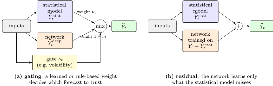
Figure 48: Two designs that sit between forecast combination and a structural hybrid. (a) A gate mixes a statistical forecast and a network forecast. (b) The network is trained on the error of the statistical model, and its output is added back. Trained separately, both are forecast combination (Section 8.5); trained together, they are hybrids. Schematic.
