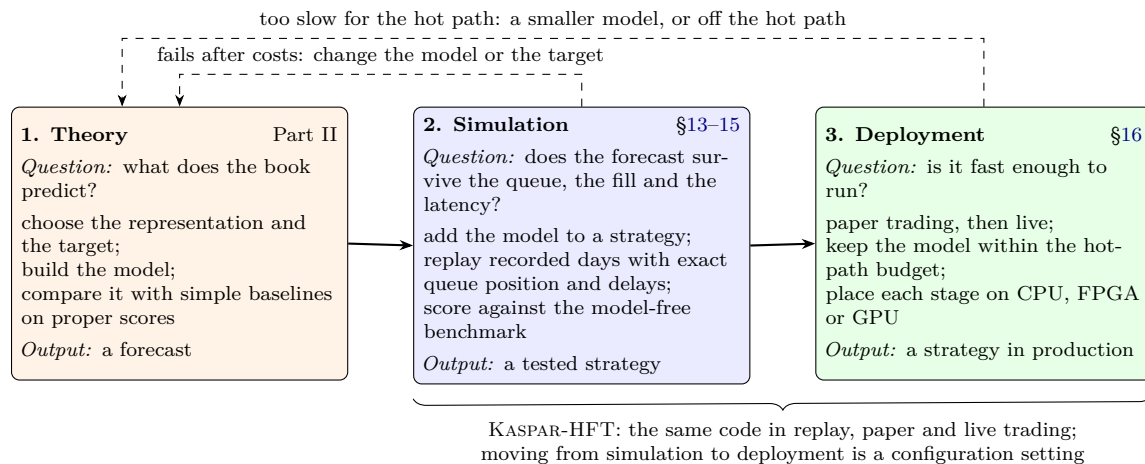
Figure 1: The path from theory to production that the survey follows. Each stage asks its own question and passes on its output only if the answer is yes; a strategy that fails in simulation, or a model too slow for the hot path, goes back to the first stage.
