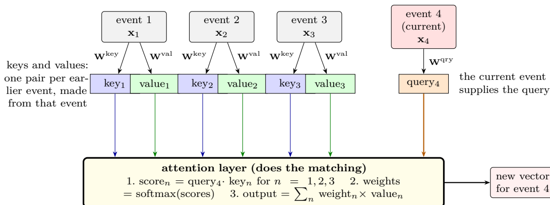
Figure 66: Attention on order-book events, for the newest event. Each earlier event is turned by learned matrices into a key (how it describes itself) and a value (what it passes on). The current event is turned into a query (what it is looking for). The attention layer scores the query against every key, converts the scores to weights, and sends the weighted average of the values back to the current event. In self-attention every event in the window takes its turn as the current one, each with its own query, against the keys and values of the events before it.
