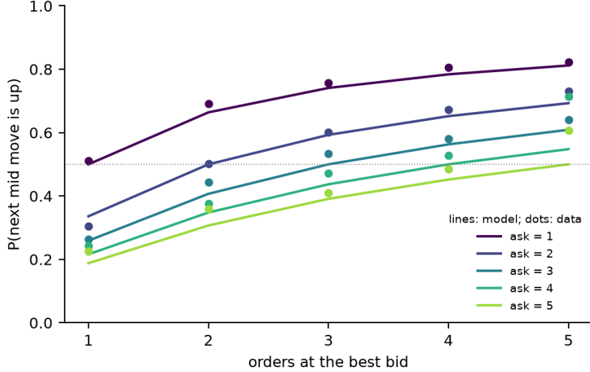
Figure 6: Probability that the next mid move is up, against the number of orders at the best bid, one curve per size of the best-ask queue: Cont–Stoikov–Talreja model (lines) and empirical frequency (dots), from Table 11. More orders at the bid, or fewer at the ask, make an up move more likely—the thin side breaks first. For large ask queues the dots sit above the lines: the model makes a large ask queue push the price down harder than it does in the data.
