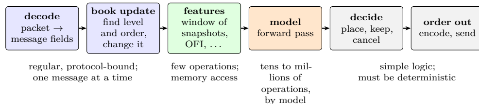
Figure 88: The per-event pipeline of a model-driven trading system. The model stage is the only one whose cost depends on the modeller’s choices. Schematic.
