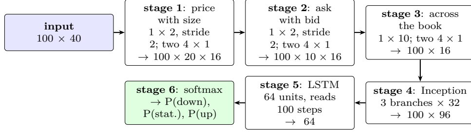
Figure 64: DeepLOB stage by stage, with the shape of the data after each stage (events \times columns \times filters). The shapes follow from the filter sizes and strides given by Zhang et al. (2019a).
