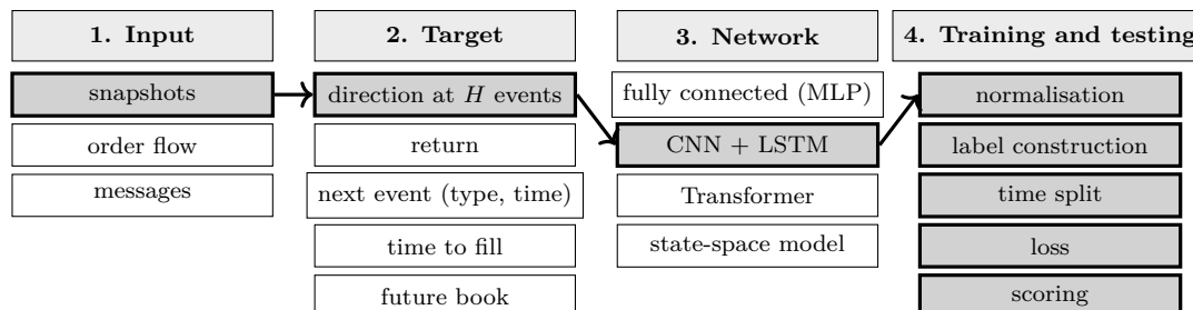
Figure 49: The four design choices of a deep LOB model. Columns 1–3: one option is chosen. Column 4: every step must be specified. Shaded with thick border: DeepLOB (snapshots; direction at 20, 50, 100 events; CNN + LSTM; previous-five-day normalisation, averaged label, 6/3/3-month split, cross-entropy, F1).
