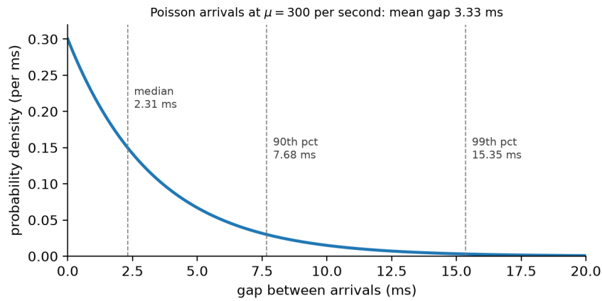
Figure 17: The exponential density of the gaps between arrivals of a Poisson process at 300 arrivals per second. Dashed vertical lines mark the median, the 90th and the 99th percentile. Half the gaps are shorter than the median of 2.3 ms and 10% are longer than 7.7 ms. Real market-data streams have far more mass near zero and a much heavier right tail. Redrawn from Maciejewski (2026b).
