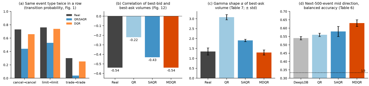
Figure 40: Results reported by Bodor and Carlier (2025) for Euro-Bund futures, re-plotted from the paper’s figures and tables; not our data. (a) Probability that an event is followed by one of the same type: the classical models cannot represent this. (b) Correlation of best-bid and best-ask volumes. (c) Shape of a gamma distribution fitted to the best-ask volume. (d) Balanced accuracy of the direction of the mid over the next 500 events; dashed line: three-class guessing.
