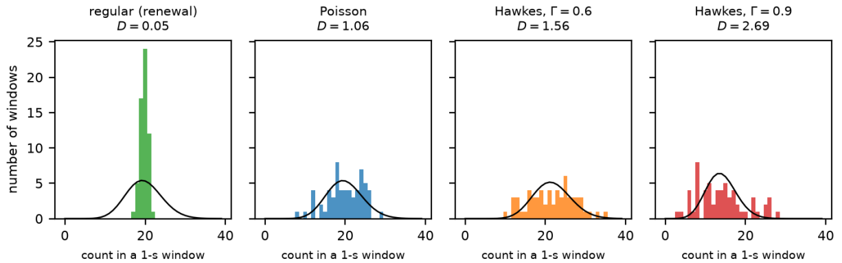
Figure 22: Distribution of arrivals per one-second window (bars) for the four processes of Figure 21, with the Poisson distribution of the same mean overlaid (curve). The regular process is far narrower than Poisson; the Poisson process matches; the Hawkes processes are wider, with extra mass in both tails. The CME NQ packet stream has D(1\text{ s}) = 108 , far wider than any panel shown ( Maciejewski, 2026b ). Stylised simulation.
