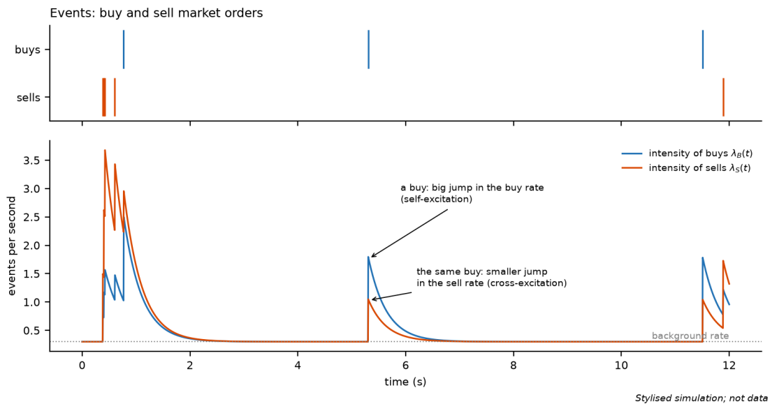
Figure 18: Intensity, self- and cross-excitation. Top: a simulated stream of buy and sell market orders. Bottom: the intensity of each. Each event makes both curves jump, by more for its own type (self-excitation) than for the other (cross-excitation); between events both decay towards the background rate (dotted). Where events come close together, as near the start, the jumps pile up and the rates climb. Two-type Hawkes process with exponential kernels; stylised simulation, not data.
