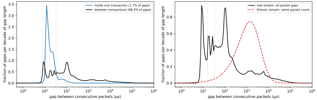
Figure 4. Packet interarrival gaps, pooled over the corpus. Left: the two packets of a split transaction arrive about 15 \mu\text{s} apart (blue: median 15 \mu\text{s} , 54% under 16 \mu\text{s} , 96% under 64 \mu\text{s} ; n = 5.6 \times 10^7 gaps), closer than a typical pair of packets from different transactions (black: median about 80 \mu\text{s} , spread from the 7.5 \mu\text{s} floor to seconds; n = 3.24 \times 10^9 gaps, 98.3% of all gaps) — but almost never as close as the floor (0.1%). Below 10 \mu\text{s} the blue curve holds 1.6% of its gaps and below 7.5 \mu\text{s} 0.1%; the region from the floor to 12 \mu\text{s} is filled by the black curve alone. So the exchange paces the pieces of one event at a steady 15 \mu\text{s} , and the tightest gaps on the feed, the ones that make a receiver queue, are between packets of different events. Right: the gap distribution of the real stream (black; the left panel’s black curve with the blue folded in) against that of a Poisson stream with the same packet count over the same window (red, dashed) — the same null as in Table 2, drawn in gap space. The Poisson density is one hump near 1 ms with a few percent of its mass below 100 \mu\text{s} ; the real density puts a third of its mass below 32 \mu\text{s} , with the edge at the floor and the mode near 100 \mu\text{s} absent from the null. The panel is the visual form of Table 5: the whole region of gaps shorter than an HFT service time is present in the real stream and absent from an independent-events stream at the same rate, which is why the uniform null carries no tail below 32 \mu\text{s} , and the 100 \mu\text{s} mode is the characteristic spacing of successive transactions within a burst, the scale on which the self-excitation of Table 6 acts. Axes: logarithmic gap axis; vertical axis the fraction of gaps per decade of gap length (twenty bins per factor of ten; the area under a curve over a range is the fraction of that curve’s gaps in the range, total area one, so heights compare shapes, not counts). Dotted lines at 7.5, 16 and 32 \mu\text{s} .
