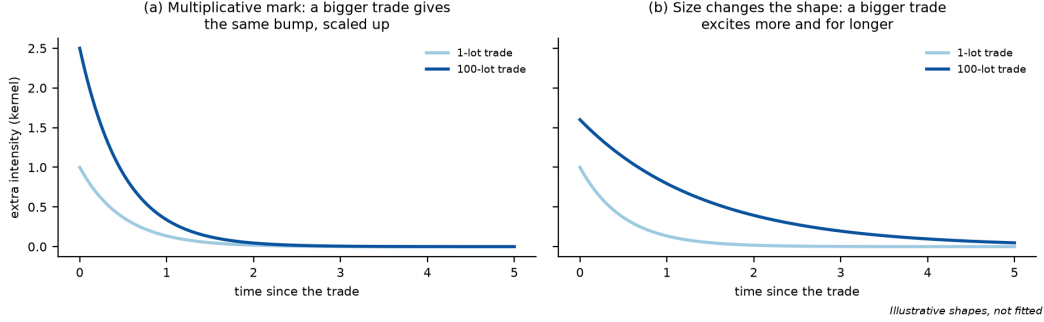
Figure 26: Two ways a trade’s size can change its effect on later events. (a) Multiplicative: the bump keeps its shape and is scaled up. (b) Non-separable: a larger trade’s bump is higher and decays more slowly. On Bund and DAX futures the data favour (b) (Rambaldi et al., 2017). Illustrative shapes, not fitted.
