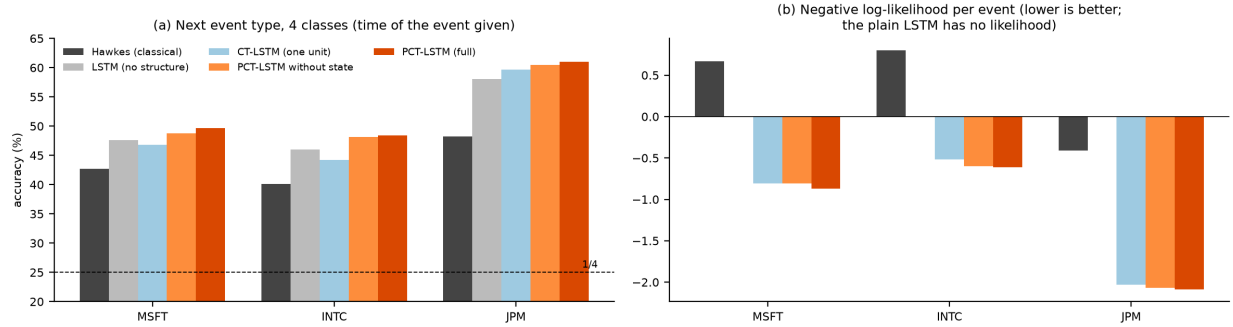
Figure 42: Results reported by Shi and Cartlidge (2022) , Table 1, re-plotted; not our data. (a) Accuracy of predicting the type of the next event, with the time of the event given; dashed line: guessing among four types. (b) Negative log-likelihood per event; the plain LSTM has no likelihood.
