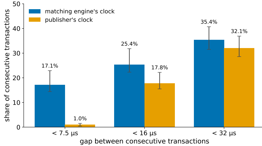
Figure 10. Table 11 as bars: share of consecutive NQ transactions closer than 7.5, 16 and 32 \mu s, on the engine's clock (blue) and the publisher's (orange); whiskers span the 40 sessions. Below 7.5 \mu s the engine has one gap in six and the publisher almost none: the publisher does not send faster than its spacing. By 32 \mu s the two clocks nearly agree.
