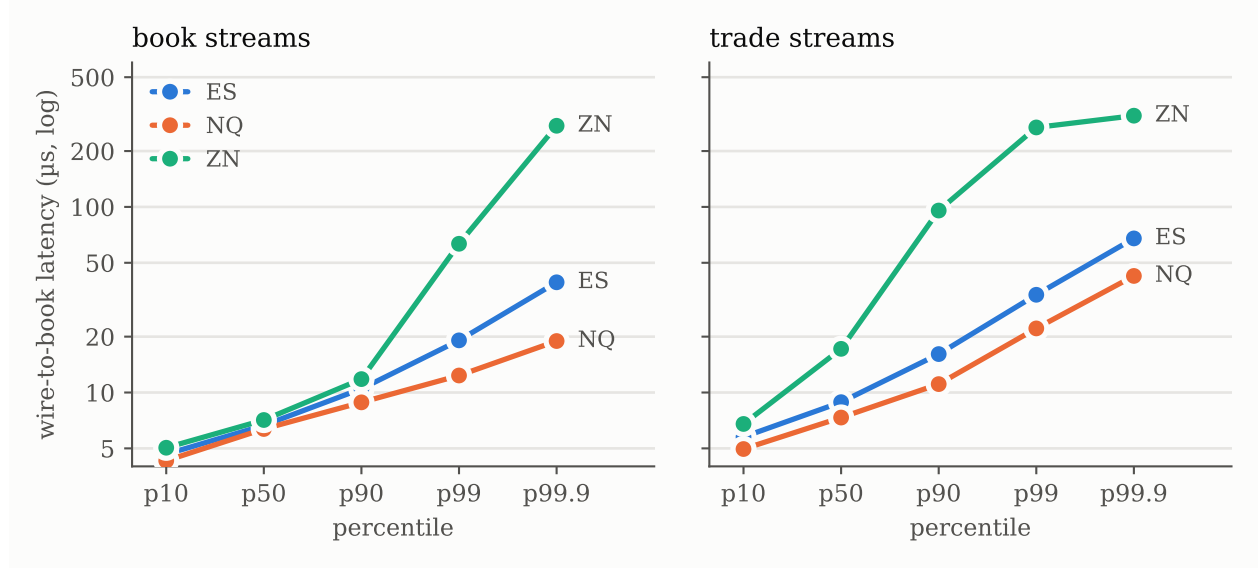
Figure 17. Serial wire-to-book latency by percentile on the six live streams, one 900 s window each, recovery excluded (book streams left, trade streams right, log latency axis). The tails order by messages per packet and cost per message, not by packet rate: the busiest stream (NQ book) has the smallest tail.
