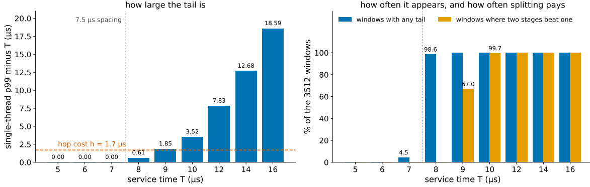
Figure 9. The table above as bars; the dotted line marks the publisher’s spacing of about 7.5 \mu\text{s} . Left: how far the single-thread p_{99} sits above the service time. Below the spacing there is no tail at all; above it the tail grows fast, and it passes the hop cost of one split ( 1.7 \mu\text{s} , dashed) between T = 8 and 9 \mu\text{s} . Right: the share of windows that have any tail (blue) jumps from 4.5% to 98.6% between 7 and 8 \mu\text{s} ; the share where two stages beat one (orange) follows about 1.5 \mu\text{s} later, once the tail is larger than the hop cost: none at 8 \mu\text{s} , two thirds at 9, all from 10 \mu\text{s} .
