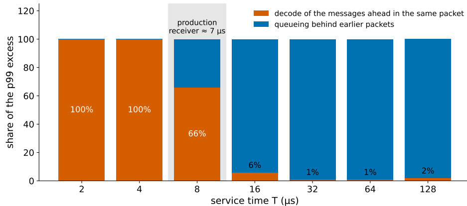
Figure 15. The decomposition above as bars: of the simulated p_{99} excess at each service time, the part due to decoding the messages ahead in the same packet (vermillion) and the part due to queueing behind earlier packets (blue). At and below the floor the decode of long packets is the tail; the shaded bar, T = 8 \mu s , is the nearest simulated service time to a production receiver’s 7 \mu s , and there it is two thirds. From 16 \mu s queueing is almost all of it.
