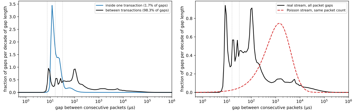
Figure 5. Packet interarrival gaps, pooled over the corpus. Left: the two packets of a split transaction arrive about 15\ \mu\text{s} apart (blue: median 15\ \mu\text{s} , 54% under 16\ \mu\text{s} , 96% under 64\ \mu\text{s} ; n = 5.6 \times 10^7 gaps), closer than the gap between consecutive packets of different transactions (black: median about 80\ \mu\text{s} , spread from the 7.5\ \mu\text{s} floor to seconds; n = 3.24 \times 10^9 gaps, 98.3% of all gaps) — but almost never as close as the floor (0.1%). Below 10\ \mu\text{s} the blue curve holds 1.6% of its gaps and below 7.5\ \mu\text{s} 0.1%; the region from the floor to 12\ \mu\text{s} is filled by the black curve alone. So the exchange paces the pieces of one event at a steady 15\ \mu\text{s} , and the tightest gaps on the feed, the ones that make a receiver queue, are between packets of different events. Right: the gap distribution of the real stream (black; the left panel's black curve with the blue folded in) against that of a Poisson stream with the same packet count over the same window (red, dashed) — the same null as in Table 2, drawn in gap space. The Poisson density is one hump near 1\ \text{ms} with a few percent of its mass below 100\ \mu\text{s} ; the real density puts a third of its mass below 32\ \mu\text{s} , with the edge at the floor and the mode near 100\ \mu\text{s} absent from the null. The panel is the visual form of Table 5: the whole region of gaps shorter than an HFT service time is present in the real stream and absent from an independent-events stream at the same rate, which is why the uniform null carries no tail below 32\ \mu\text{s} , and the 100\ \mu\text{s} mode is the characteristic spacing of successive transactions within a burst, the scale on which the self-excitation of Table 6 acts. Axes: logarithmic gap axis; vertical axis the fraction of gaps per decade of gap length (twenty bins per factor of ten; the area under a curve over a range is the fraction of that curve's gaps in the range, total area one, so heights compare shapes, not counts). Dotted lines at 7.5 , 16 and 32\ \mu\text{s} .
