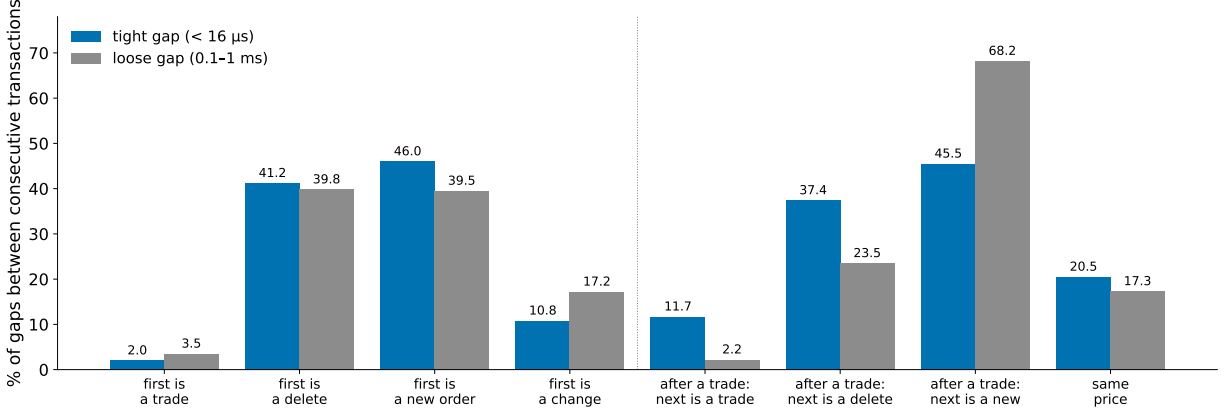
Figure 14. Table 17 as bars: the kind of transaction on either side of a tight gap (blue, under 16 \mu s) and of a loose gap (grey, 0.1–1 ms). Left of the dotted line the two mixes are alike: tight gaps are ordinary quote traffic. Right of it, after a trade the next transaction is far more often another trade or a delete across a tight gap, the pattern a race would leave.
