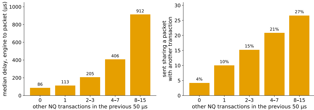
Figure 12. Table 13 as bars. Left: median delay from engine to packet grows tenfold as the engine gets busier. Right: the share of transactions sent in a packet with another transaction grows from 4% to 27%. Both rising together is what a queue at the publisher looks like.
