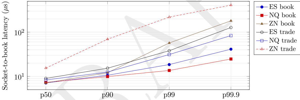
Figure 4. Socket-to-book latency percentiles per stream (Table 10), log scale. Medians cluster near 7\text{--}15 \mu\text{s} ; the tails diverge, ZN trade reaching 219 \mu\text{s} at p99 and 410 \mu\text{s} at p99.9 .
