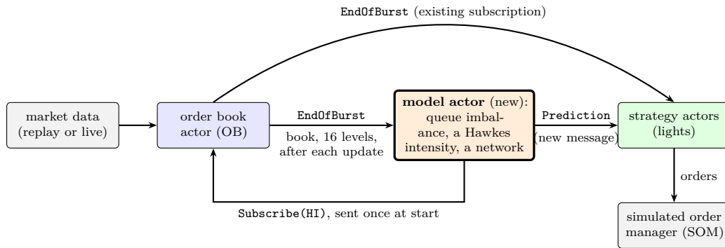
Figure 79: An order-book model added to Kaspar as an actor. It subscribes to the order book, receives the book after each burst of updates, and sends a prediction message to each strategy actor. Message names are those in the code; the model actor, the Prediction message and its handler in the strategy are new.
