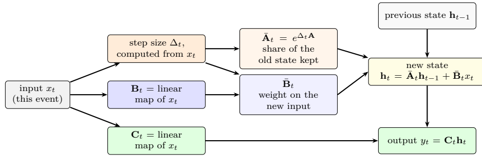
Figure 74: One step of Mamba’s selective state-space layer. The current input sets the step size \Delta_t and the matrices \mathbf{B}_t and \mathbf{C}_t ; the step size sets how much of the previous state survives. After Gu and Dao (2024).
