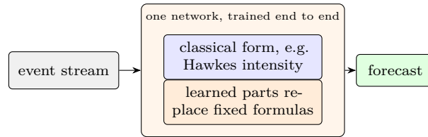
(b) structural hybrid : classical structure inside the learner
