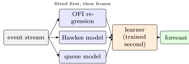
(a) meta-model : classical models outside, the learner sees only their outputs
