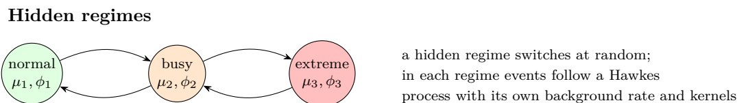
Figure 28: A Markov-modulated Hawkes process with three regimes. The regime is not observed; it is inferred from the pattern of events. Schematic.
