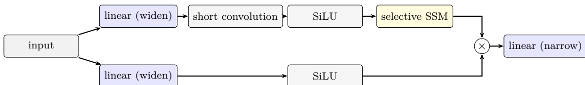
Figure 75: The Mamba block. The second branch gates the output of the selective state-space layer by multiplication. After Gu and Dao (2024).
