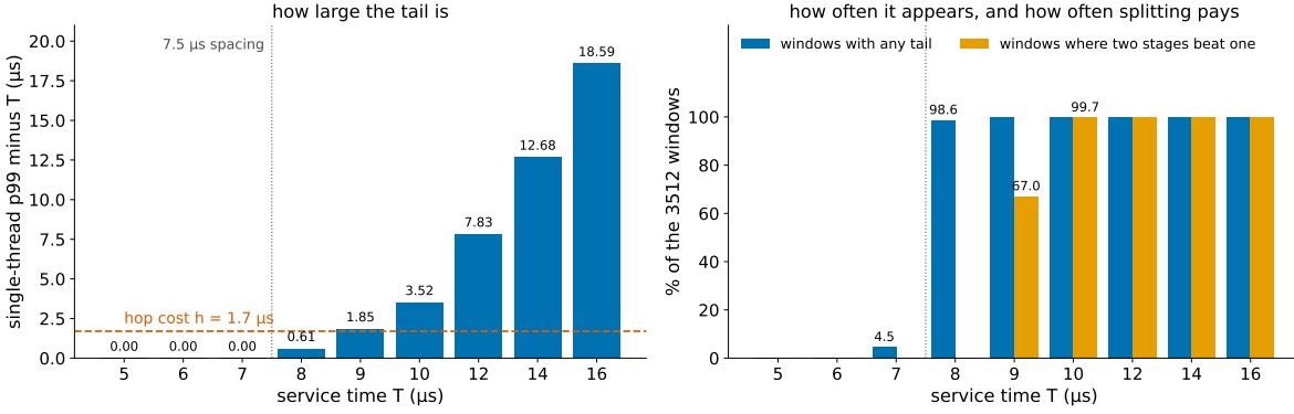
Figure 13. The table above as bars; the dotted line marks the publisher spacing of about 7.5\ \mu\text{s} . Left: how far the single-thread p_{99} sits above the service time. Below the spacing there is no tail at all; above it the tail grows fast and passes the hop cost of one split (dashed) between 8 and 9\ \mu\text{s} . Right: the share of windows that have any tail (blue) jumps from almost none to almost all between 7 and 8\ \mu\text{s} ; the share where two stages beat one (orange) follows about 1.5\ \mu\text{s} later, once the tail is larger than the hop cost.
