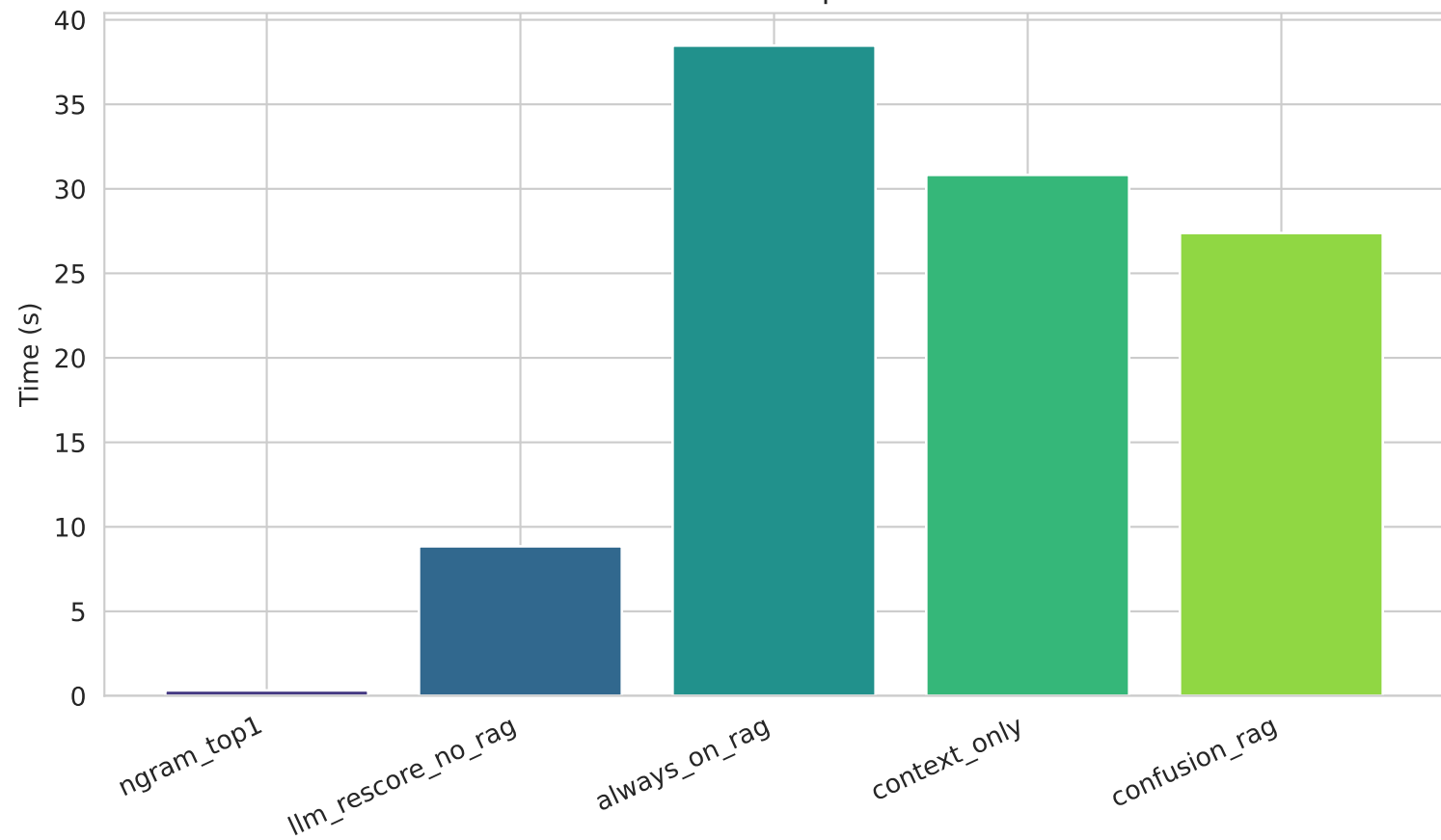
Runtime Comparison
