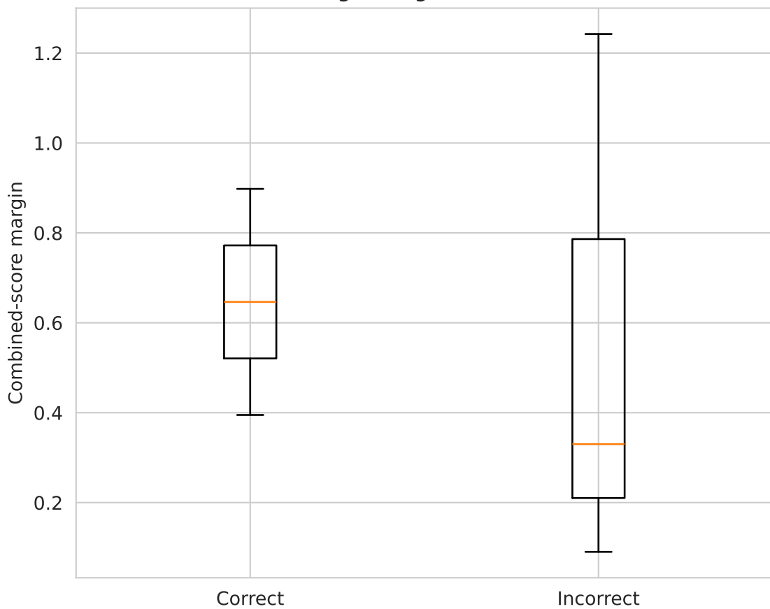
LLM Change Margin vs Correctness
