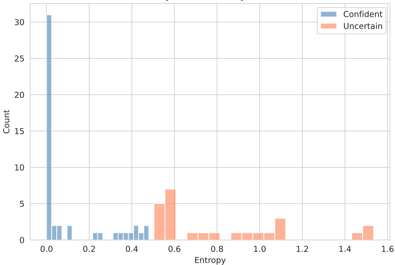
Uncertainty Distribution by Gate Result
