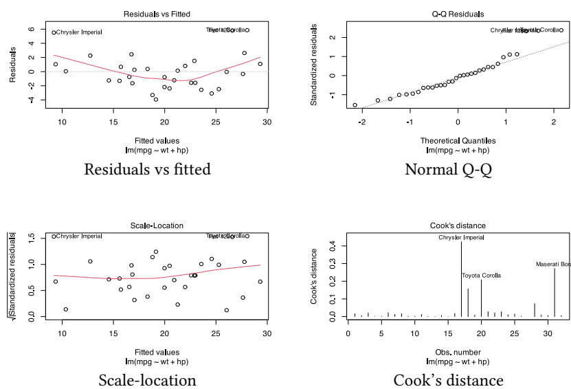
Figure 4: Regression diagnostics
