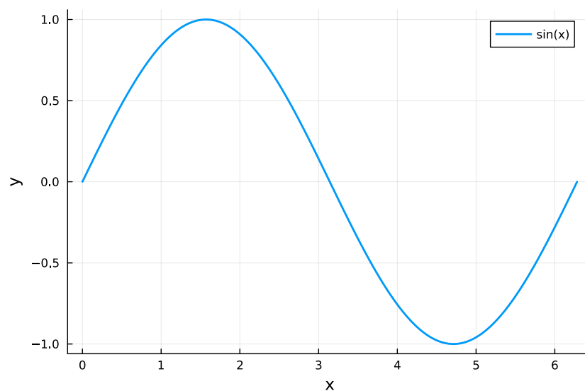
Figure 3: Julia sine wave
