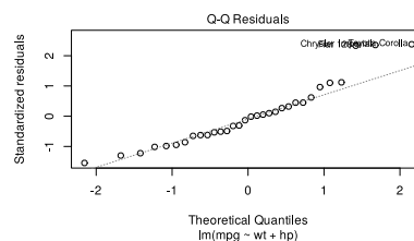
(b) Normal Q-Q
