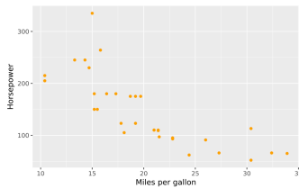
Figure 1: Plotnine scatterplot
