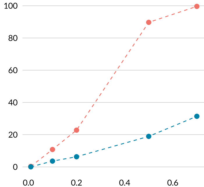
Statistical Power (%)
