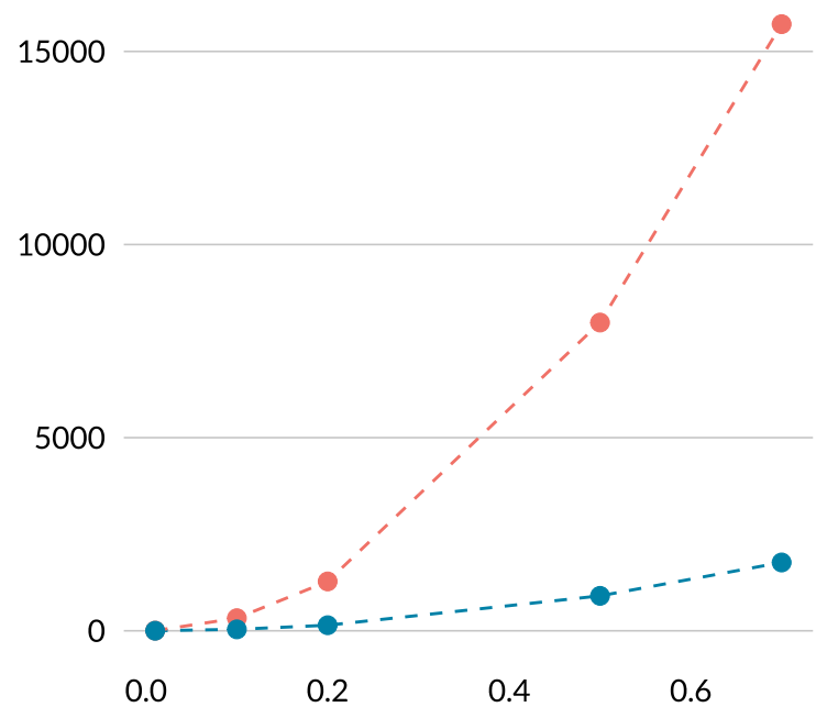
F-Statistic
