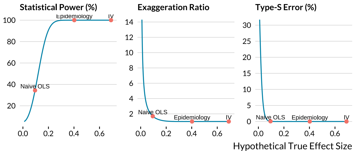
Figure B.1: Power, Exaggeration and Type S Errors Curves for Deryugina et al. (2019) .
