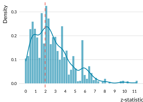
Weighted Distribution of the z-statistics More mass around the 1.96 threshold
