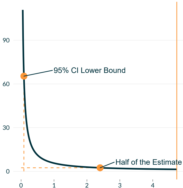
Type-M Error (Exaggeration Ratio)
